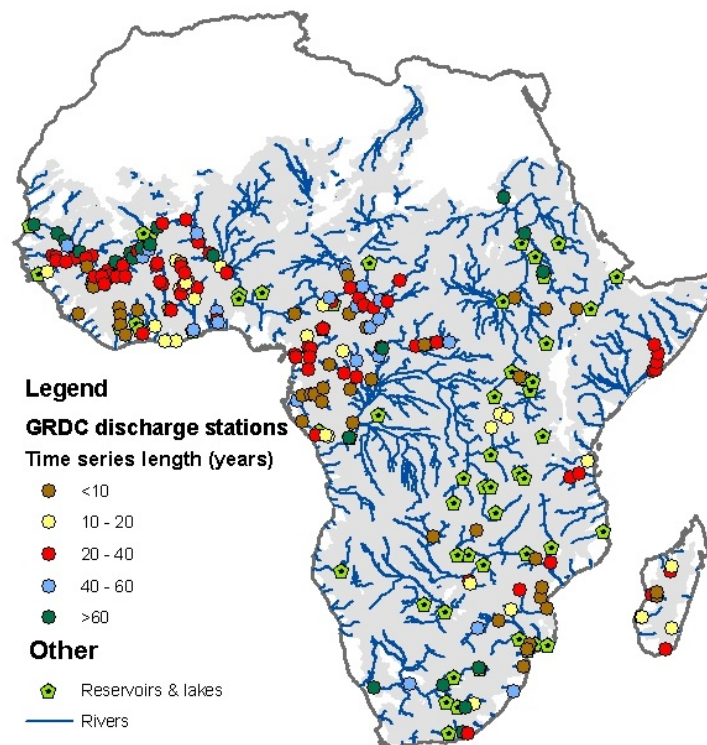
Fig. 1. Global Runoff Data Centre (GRDC) stations and reservoirs/lakes included in the SWAT-SSA model setup and calibration (Fig. 2 in the manuscript)
