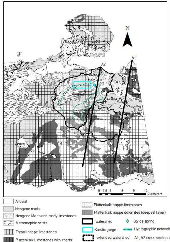
Fig. 1. Geology of Koiliaris River Basin.
