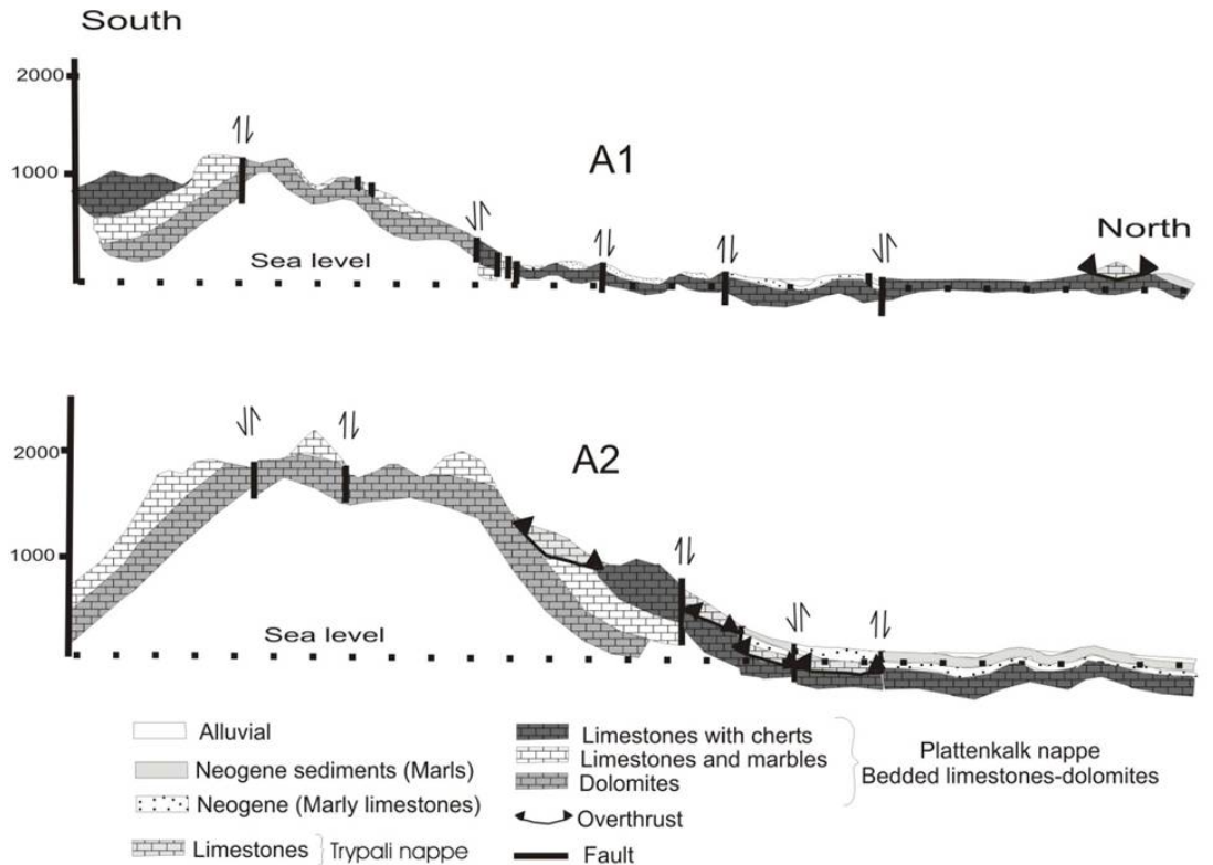
Fig. 2. Geologic cross sections of Koiliaris River Basin.
