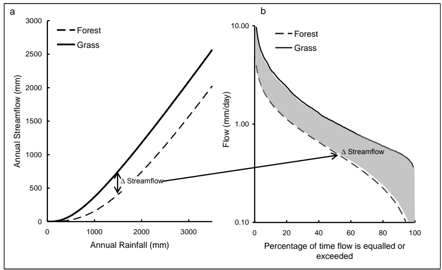
Fig. 2. Linking mean annual streamflow estimated using the method of Zhang et al. (2001) to the FDC.
