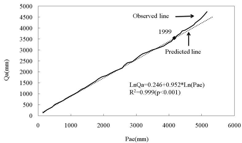
Fig. 7. Modified double mass curve.
