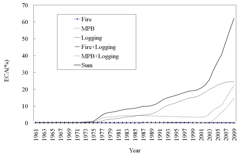
Fig. 6. Cumulative equivalent clear-cut area (ECA) from 1961 to 2009.
