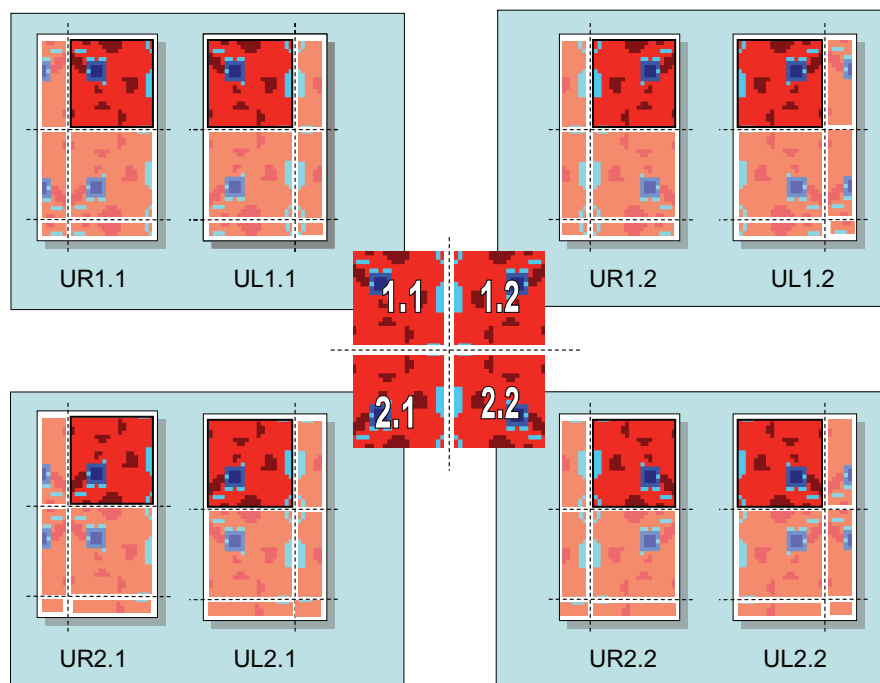
Fig. 1. Method to map initial spatial throughfall pattern of Huewelerbach on the Panola hillslope. In the center the four initial patterns. Each initial pattern can be mapped on the hillslope in two ways: the 'Upper Right' configuration (UR) and the 'Upper Left' configuration (UL).
