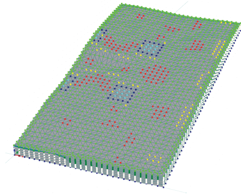
Fig. 4. Input pattern 'Upper Right-2.1' on Panola hillslope with highest impact on subsurface outflow compared to uniform input.
