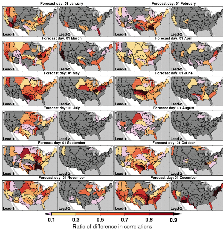
Fig. 6. The ratio of actual improvement and potential improvement in baseline runoff forecast skill at leads 1–2 months. (Dark grey color shows the sub-regions where either the potential improvement in skill is < 0.1 or the skill of OBS_Merged_ESP is not significant at 95 % significance level.)
