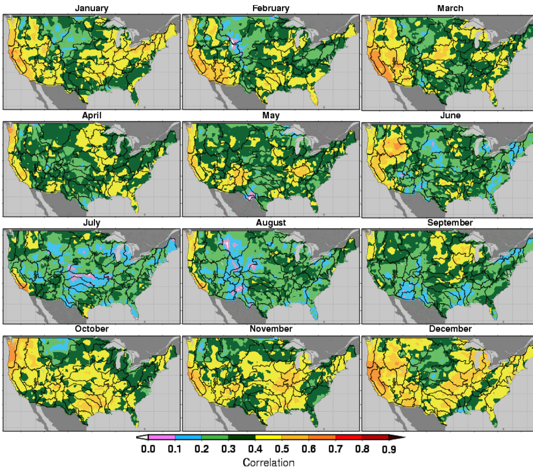
Fig. 2. Correlation between observed and forecasted (MRF) 14-day accumulated precipitation during each month.
