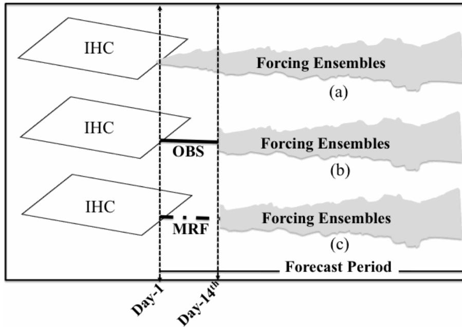
Fig. 1. Schematic showing the climate forecast framework for (a) Experiment-1 (ESP) (b) Experiment-2 (OBS_Merged_ESP) and (c) Experiment-3 (MRF_Merged_ESP).
