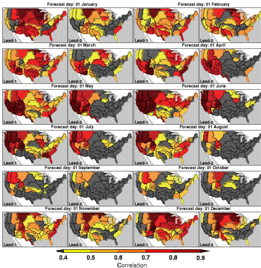
Fig. 4. Baseline skill (i.e., skill of ESP experiment) for runoff forecasts at leads 1–2 months. (Dark grey color shows the sub-regions where the baseline skill is not significant at 95 % significance level.)
