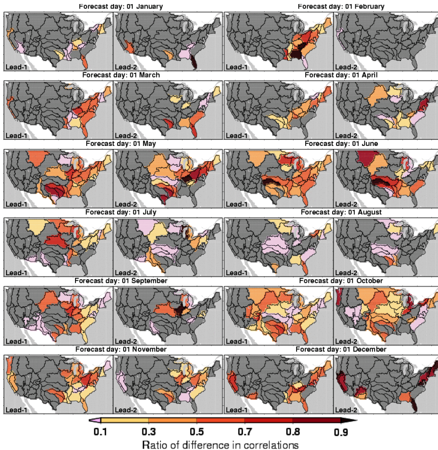
Fig. 9. The ratio of actual improvement and potential improvement in baseline SM forecast skill at leads 1–2 months. (Dark grey color shows the sub-regions where either the potential improvement in skill is <0.1 or the skill of OBS_Merged_ESP is not significant at 95 % significance level.)
