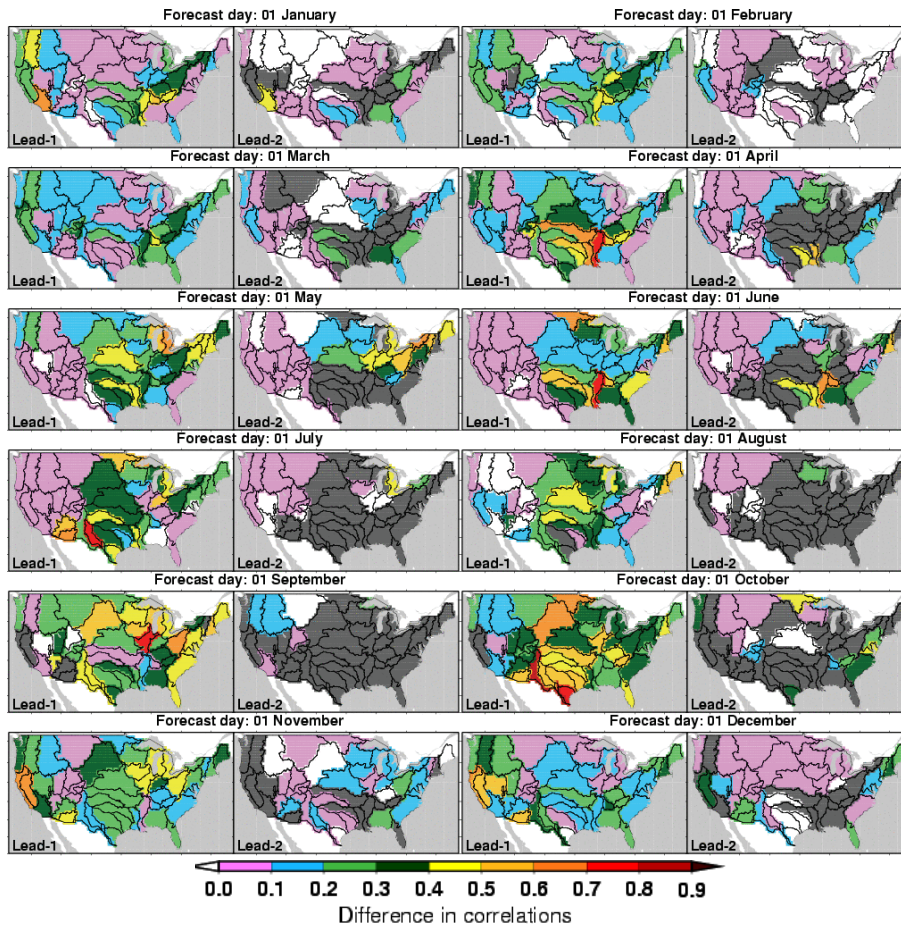
Fig. 5. Potential improvement in runoff forecast skills at leads 1–2 months. (Dark grey color shows the sub-regions where the skill of OBS_Merged_ESP is not significant at 95 % significance level.)
