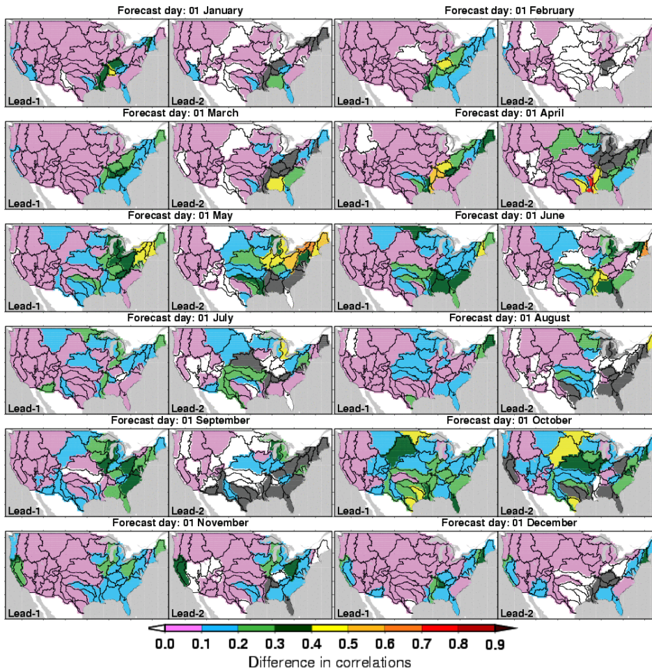
Fig. 8. Potential improvement in SM forecast skills at leads 1–2 months. (Dark grey color shows the skill of OBS_Merged_ESP is not significant at 95% significance level.)
