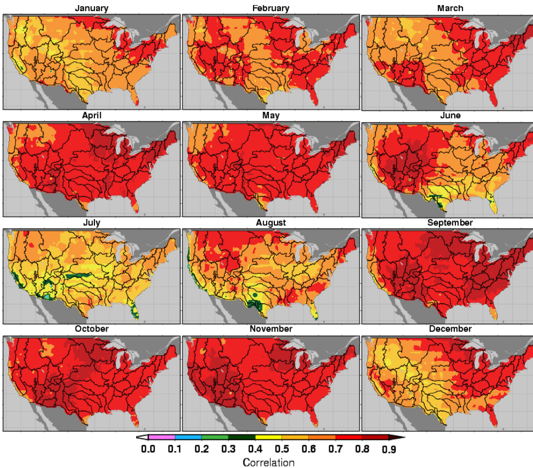
Fig. 3. Correlation between observed and forecasted (MRF) 14 days mean average daily temperature during each month.
