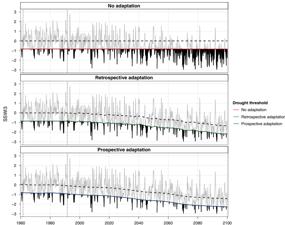
Fig. 1. Evolution of SSWI3 for a grid cell near Toulouse under the A1B scenario, and corresponding adaptation scenarios. Black filled areas correspond to local-scale drought events reaching the 20% threshold. The dashed lines show the drought index baseline evolutions calculated for each adaptation scenario and described in Table 3. Coloured lines show the corresponding drought state threshold (see text for details). The reference period is framed by dashed vertical lines.
