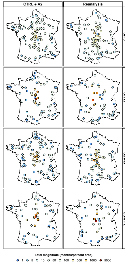
Fig. 5. Centroid of drought events identified over the 1958–2008 period, from the reanalysis (right) and from the (CTRL + A2) ARPEGE run. Colors denote different classes of total magnitude. The different rows show all four drought indices.
