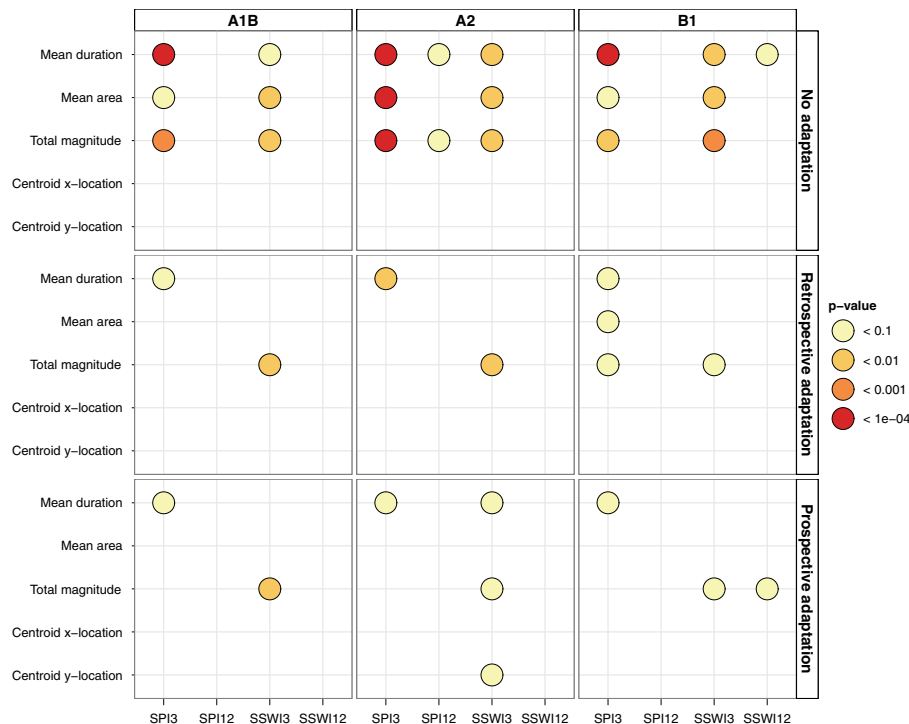
Fig. 11. Significance of the Mann-Kendall trend test (represented with the test p-value) on all combinations of drought indices and spatio-temporal characteristics, for the 3 emissions scenarios (columns) and for the 3 adaptation scenarios (lines).
