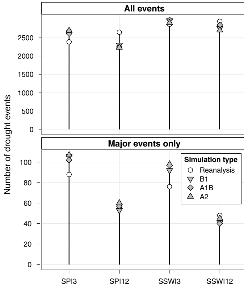
Fig. 3. Number of drought events identified over the 1958–2008 period, for reanalysis data and all 3 simulations. Top: all events; Bottom: only major events (duration > 1 month).
