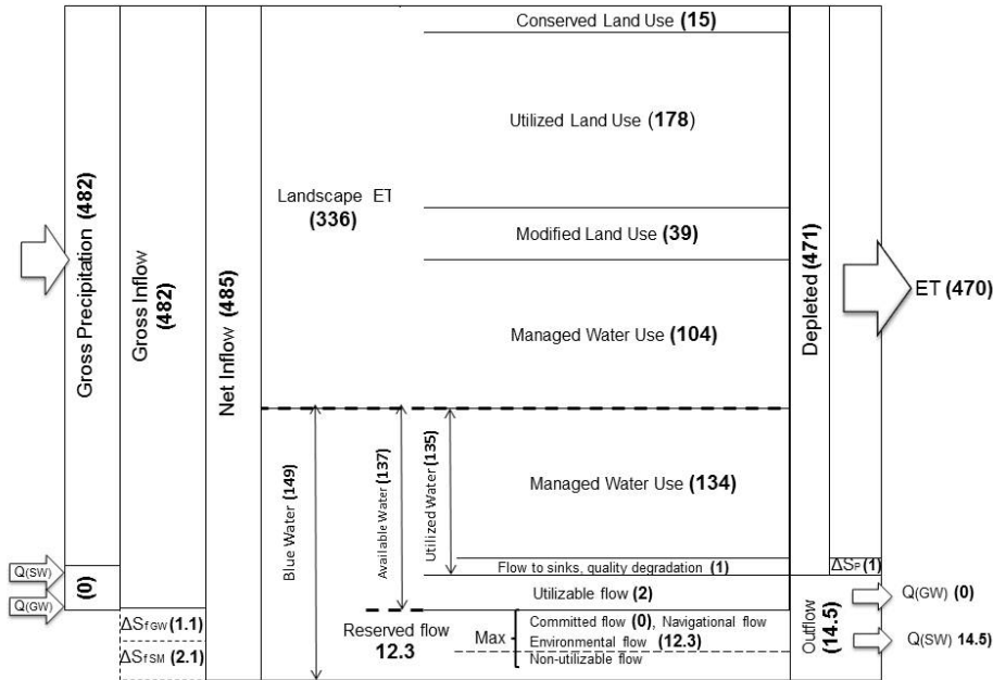
Fig. 7. Impact of scenario B on WA+ resource base sheet for the Indus. All components are in \text{km}^3 .
