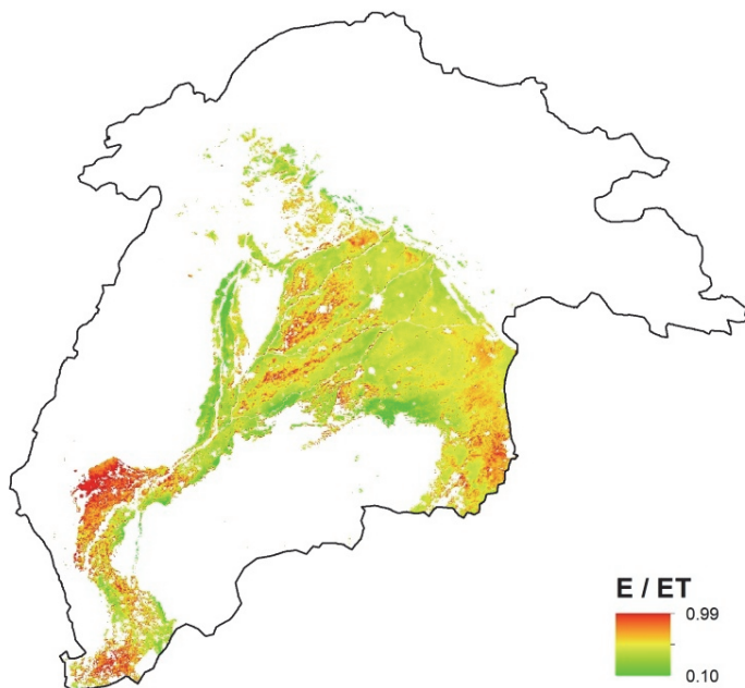
Fig. 6. Ratio of E over ET in irrigated areas of the Indus basin.
