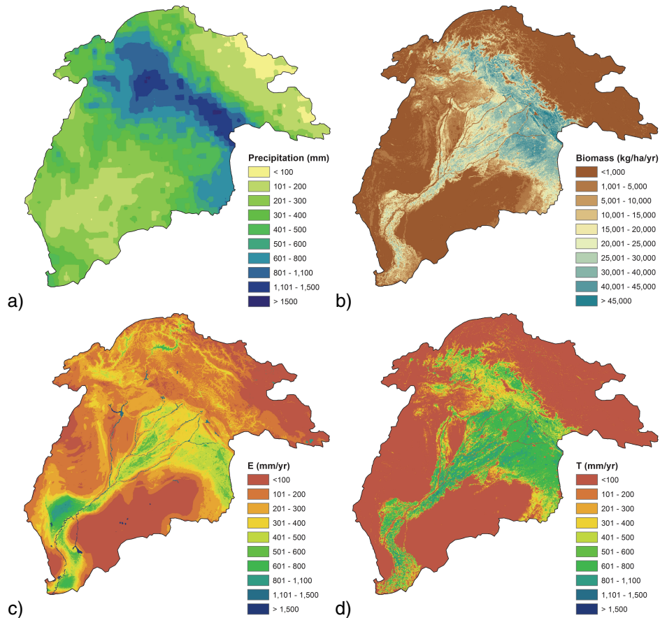
Fig. 1. (a) Precipitation (based on data from Cheema and Bastiaanssen, 2012) (b) biomass (c) evaporation (d) transpiration (based on data from Bastiaanssen et al., 2012) in the Indus Basin.
