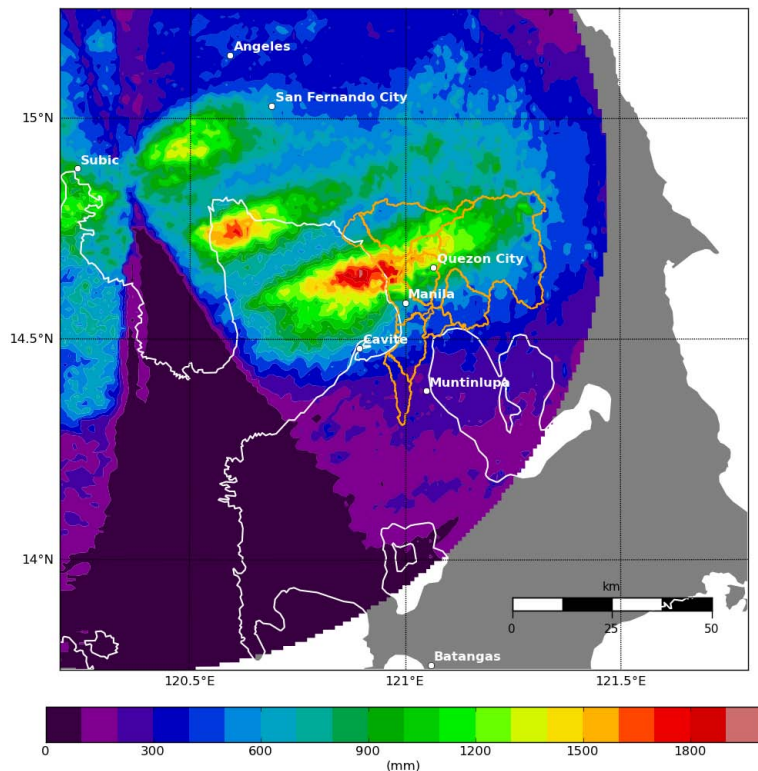
Fig. 3. Rainfall accumulation for Manila Metropolitan region, Philippines, from 6–9 August 2012, based on the S-band radar located near Subic, using wradlib modules io (reading NetCDF data), georef (geo-referencing), clutter (clutter identification), ipol (gap filling), adjust (for mean field bias adjustment), and vis (for plotting over a map). The orange lines indicate watersheds draining to Manila Metropolitan region. Note that the southern sectors of the radar exhibit significant beam shielding caused by Mount Natib, a volcano and caldera complex located in the province of Bataan.
