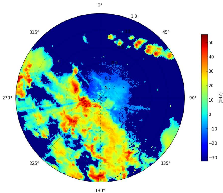
Fig. 2. Simple diagnostic plot of polar reflectivity.
