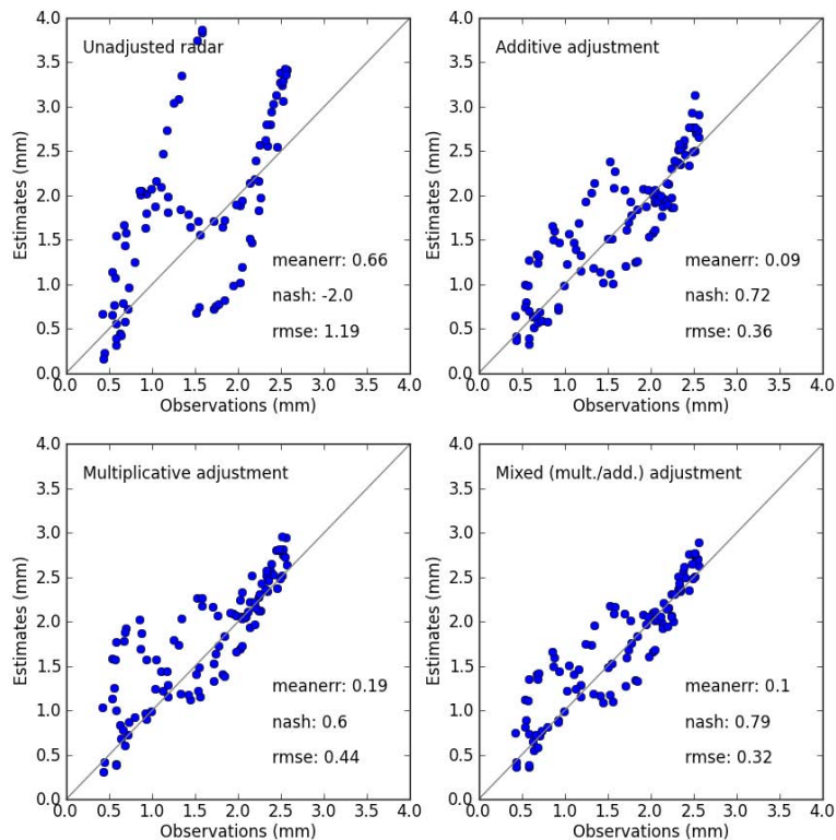
Fig. 6. Verification of the adjustment techniques, using the example shown in Fig. 5. The scatter plot and the error metrics were created using wradlib.verify . The metrics are computed by comparing the unadjusted and the adjusted radar observations against the synthetic true rainfall (just a small selection of error metrics is shown here).
