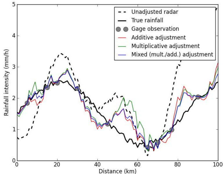
Fig. 5. A 1-D example with synthetic data for illustrating different adjustment approaches in wradlib . The true rainfall was generated by combining a sine curve with white noise. Contaminating the true rainfall with spatially variable additive and multiplicative error terms yields the unadjusted radar observation. Three adjustment methods are then applied via wradlib.adjust-0 using the gauge observations (grey circles) which are random samples of the true rainfall. See Fig. 6 for a verification of this example adjustment.
