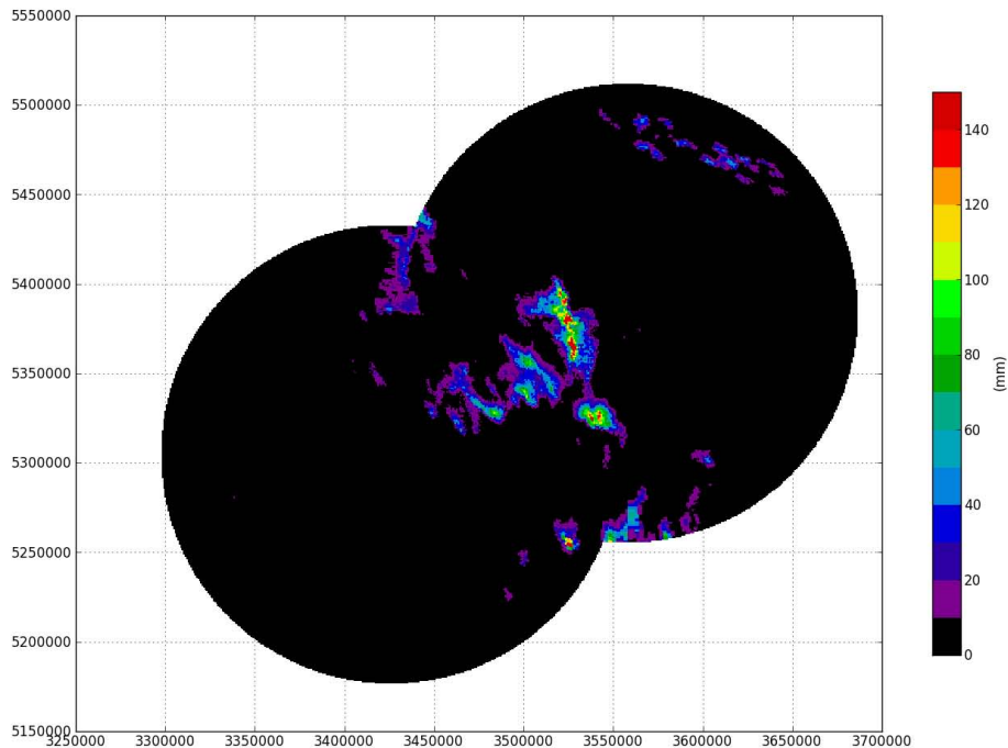
Fig. 4. Composite of a 2-h event accumulation of clutter and attenuation corrected data for 2 June 2008, 16:00–18:00 UTC, including the German Weather Service’s C-band radars Tuerkheim and Feldberg. This event caused a disastrous flash flood in the central map region.
