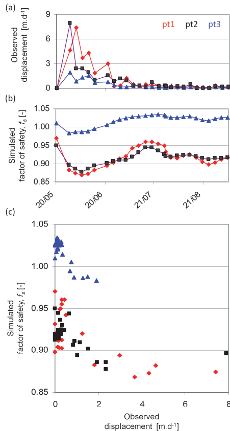
Fig. 9. (a) Observed displacement rates for points pt1, pt2 and pt3 (Travelletti et al., 2012); (b) the factor of safety, f_s , simulated with additional adjustment of “snow pack/snow melt” model; (c) the relationship between the “new” f_s and observed displacement rates (Travelletti et al., 2012). For the location of the points see Fig. 2a.
