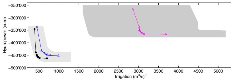
Fig. 3. IPF under historical inflow 1967-1980 (black dots), backcast 1961-1990 (blue triangles) and forecast 2071-2100 (magenta triangles) inflow scenario by RACMO-RCM.
