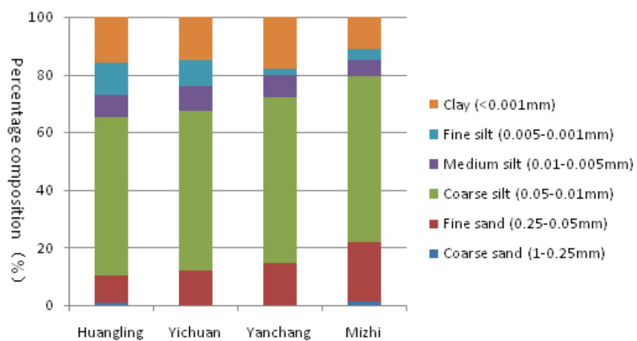
Fig. 2. Supplement figure 2 the composition of soil particle size in the northern Shaanxi Province (Zhang, 2002)
