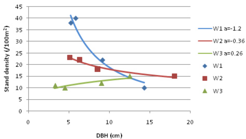
Fig. 4. Supplement figure 4 logarithmic regression between plant size and density
