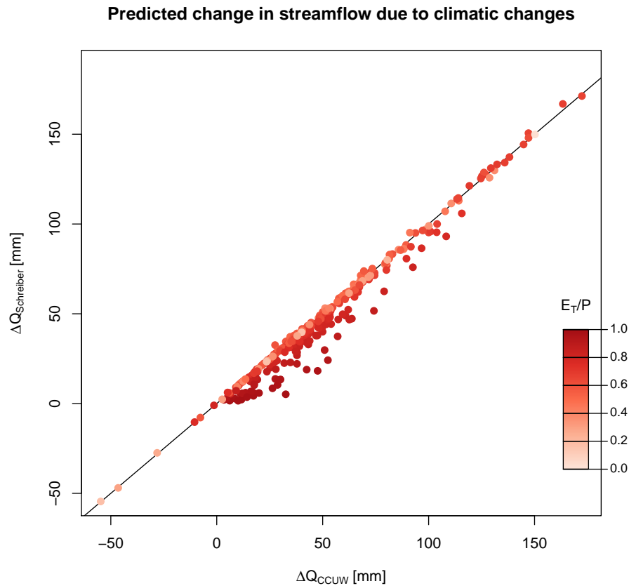
Fig. 2. Scatterplot of predicted streamflow changes of CCUW vs. Schreiber.
