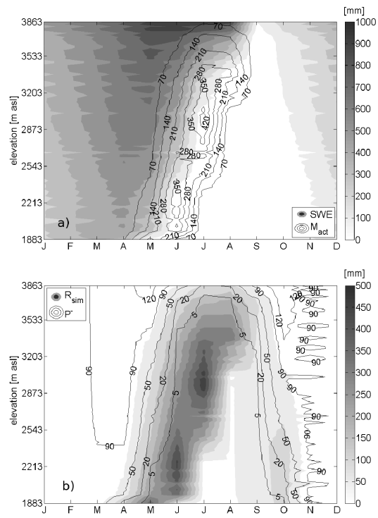
Fig. 2. Effects of elevation distribution on runoff production – River Savara at Eau Rousse. a) SWE present in the snow storage and snowmelt, M_act; b) Snowfall, P-, and runoff, R
