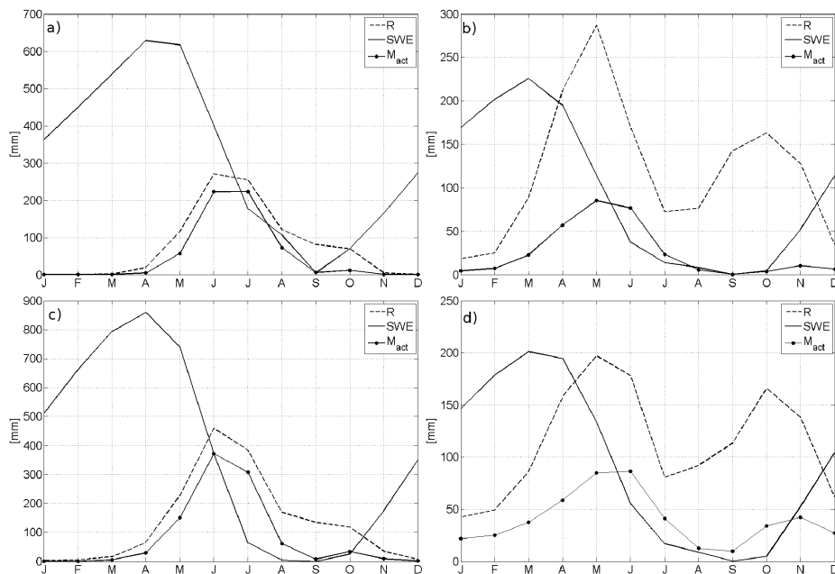
Fig. 1. Average regimes of runoff, R, snow water equivalent in the snow storage, SWE, and actual snowmelt, M_{act} . a) Savara at Eau Rouse; b) Sesia at Ponte Aranco; c) Rutor at Promise; d) Toce at Candoglia
