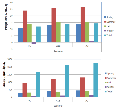
Fig. 3. Summary of forecasted temperature and precipitation results
