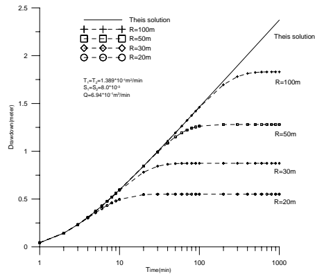
Figure B Temporal drawdown distributions predicted by the Theis solution and the present solution for different value of R .
