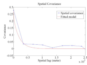
Fig. 2 Covariance values obtained from the fitted and the experimental models based on the residuals from ANFIS. (Fig. 5 of the revised manuscript)
