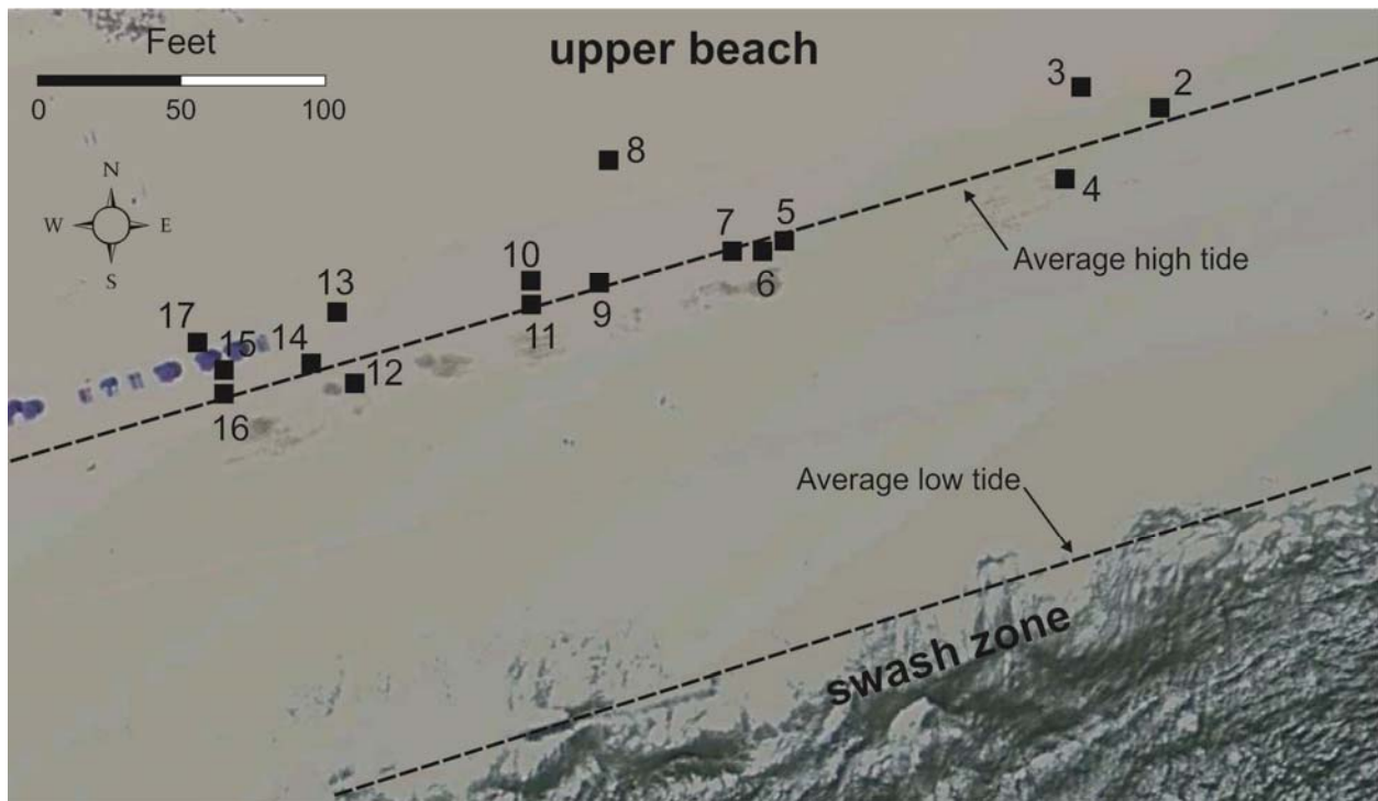
Figure 5. OSAT 1 sampling locations 2-17 along Alabama's beaches where unqualified total PAHs were observed (see Figure 1 also).
