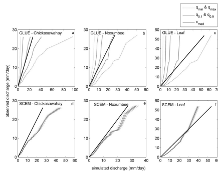
Figure 4: The joint distribution of the lowest ( q_{\min} ), highest ( q_{\max} ), 10 th ( q_{0.1} ), and 90 th ( q_{0.9} ) quantiles, and the median ( x_{\text{med}} , or 50 th quantile) of the discharge ensembles and the observations from the (a-c) GLUE and (d-f) SCEM parameter estimation methods for select sites. The solid black line in the figures is the 1:1 line and indicates perfect correlation between the simulated and observed discharge.
