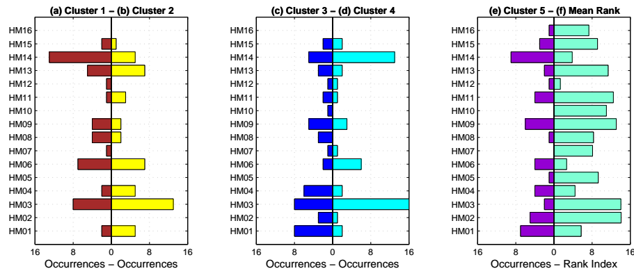
Fig. 7. Hydrological Models participation.
