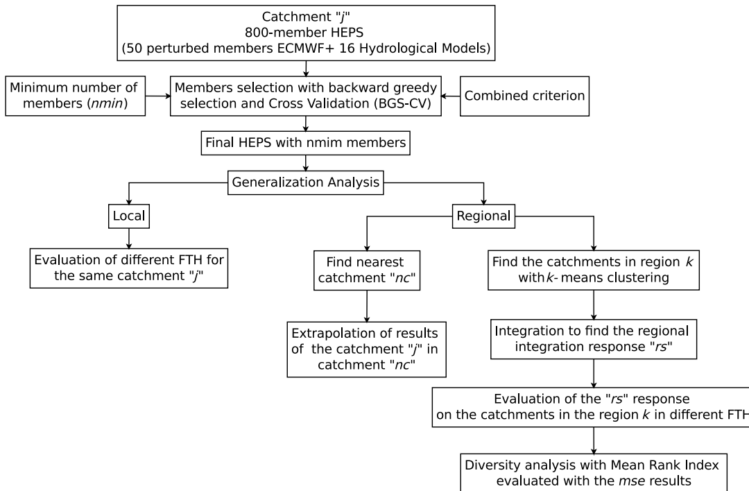
Fig. 2. Generalization of members' selection with BGS-CV.
