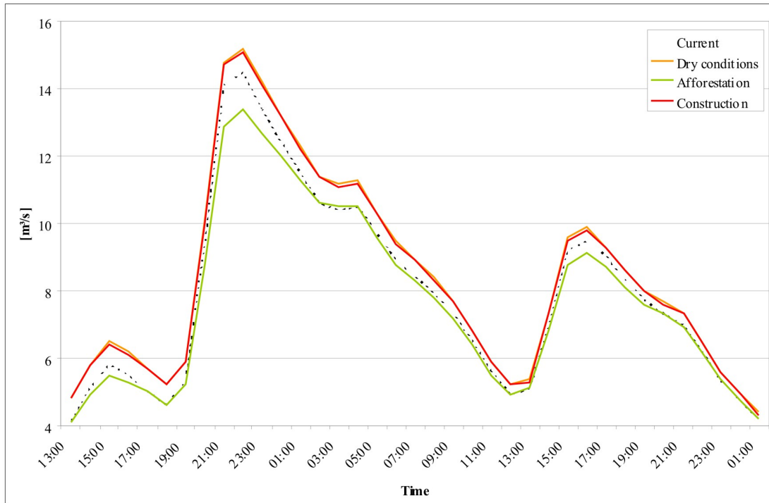
Fig. 4. Hydrograph for the different LULC patterns for the rainfall event in September 2009
