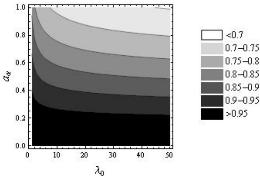
Fig. 1. Sensitivity of the quantile ratio, i.e. ratio between the quantiles with the base and seasonal distribution for a given return period, to variations of \lambda_0 (x-axis) and a_\alpha (y-axis)
