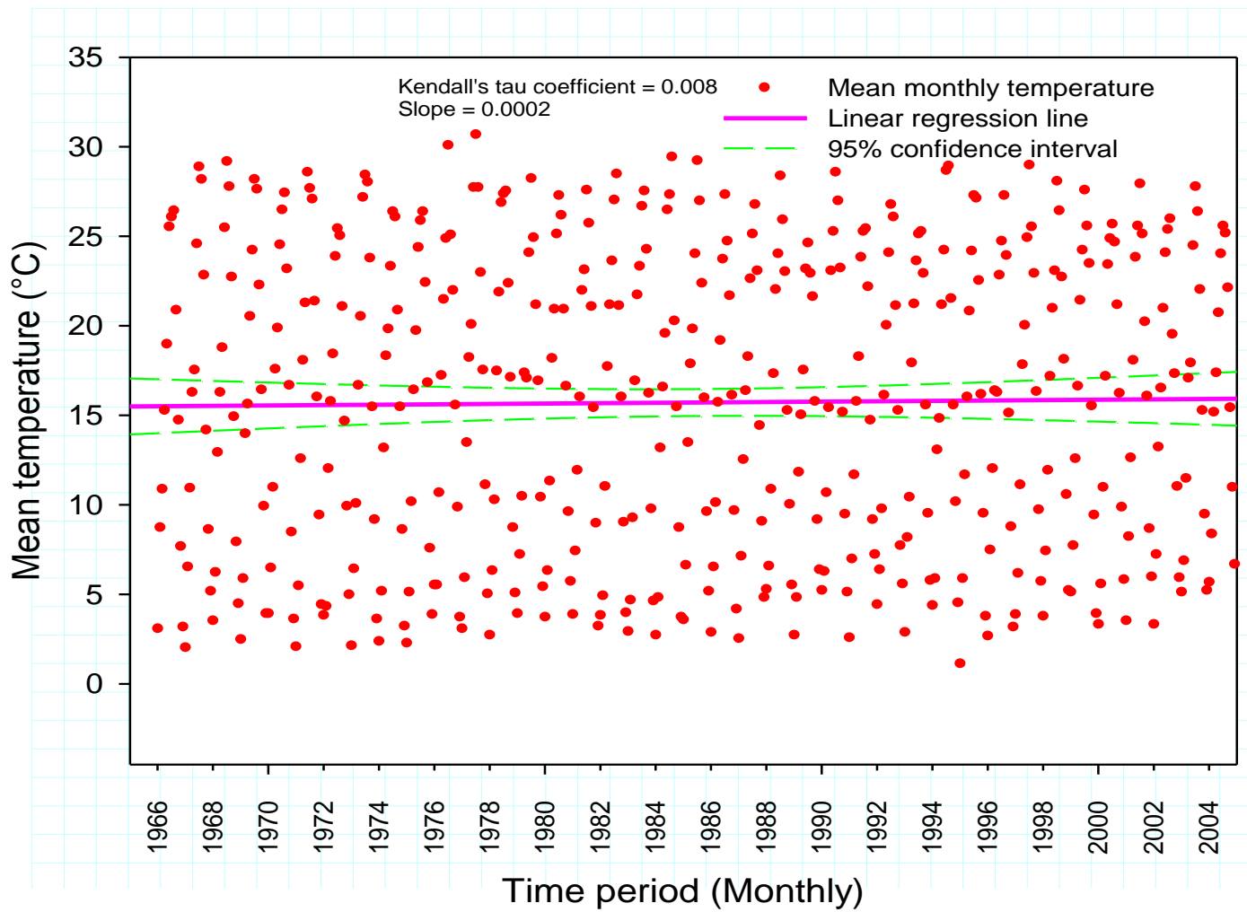
Mean temperature trend (1966-2004) on Gilgit climate station
