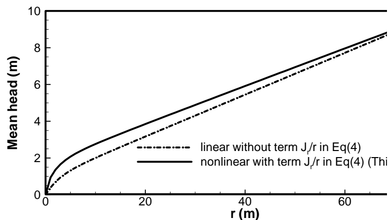
Figure: The mean head distribution for fixed z ( z=10\text{m} ) and along r -direction for cases with and without nonlinear terms in equation
