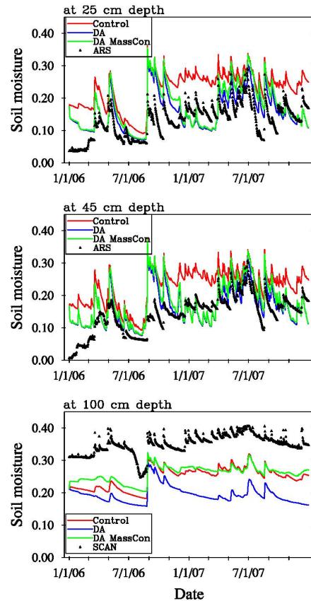
Fig. 4. Comparison of basin averaged daily soil moisture from Control, DA, and DA MassCon, interpolated at 25, 45 and 100 cm depths, with measurements from ARS stations and the SCAN site.
