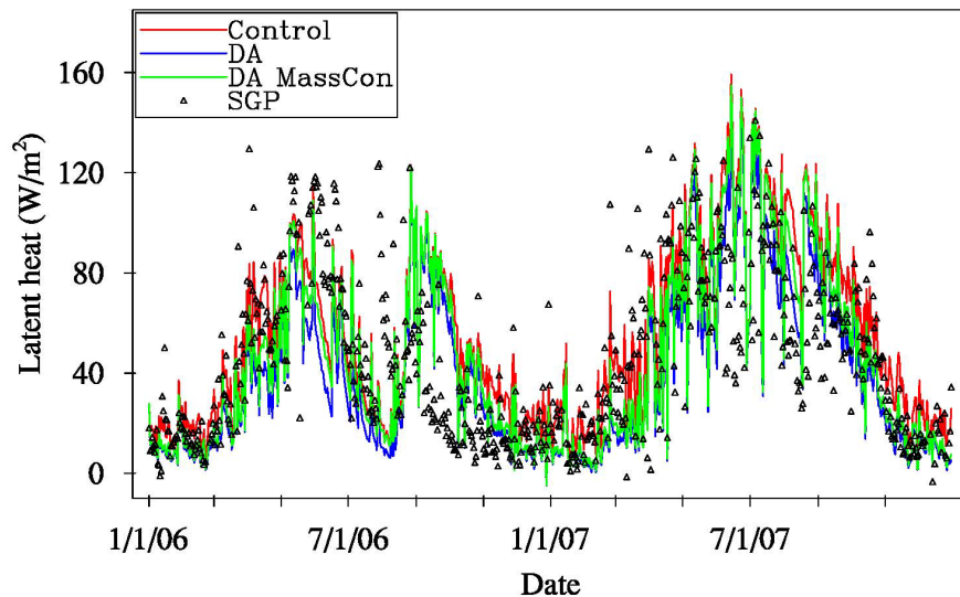
Fig. 7. Comparison of daily latent heat from Control, DA, and DA MassCon versus the SGP flux data. The daily latent heat estimates are averaged values from 6 a.m. to 6 p.m. local time for both the SGP measurements and Noah estimates.
