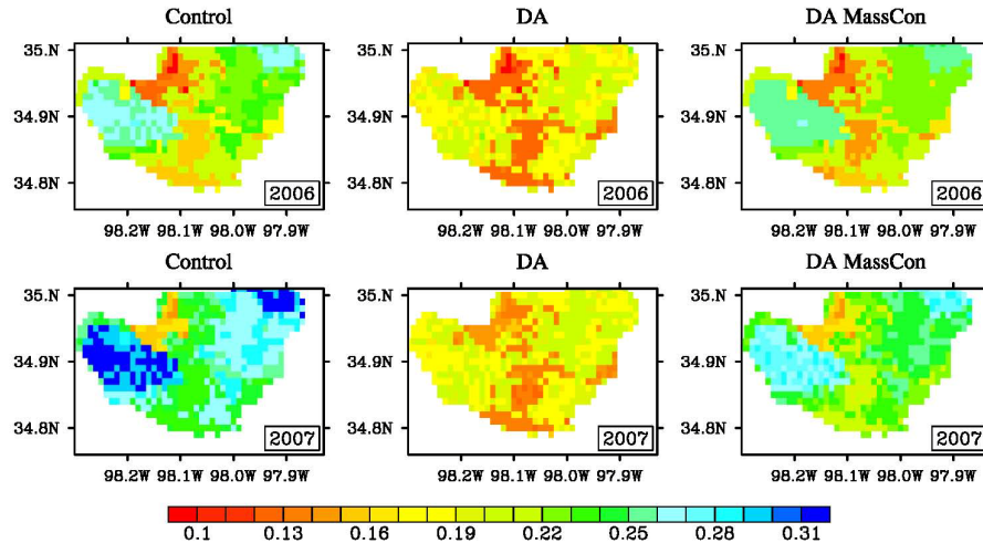
Fig. 6. Mean root zone (upper 100 cm) soil moisture from Control, DA and DA MassCon in 2006 and 2007.
