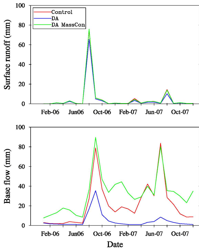
Fig. 8. Monthly surface and base flow (mm) from Control, DA and DA MassCon.
