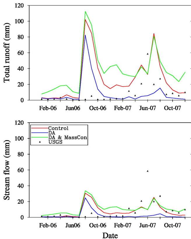
Fig. 9. Comparison of monthly total runoff and stream flow from Control, DA and DA MassCon versus USGS gauge data.
