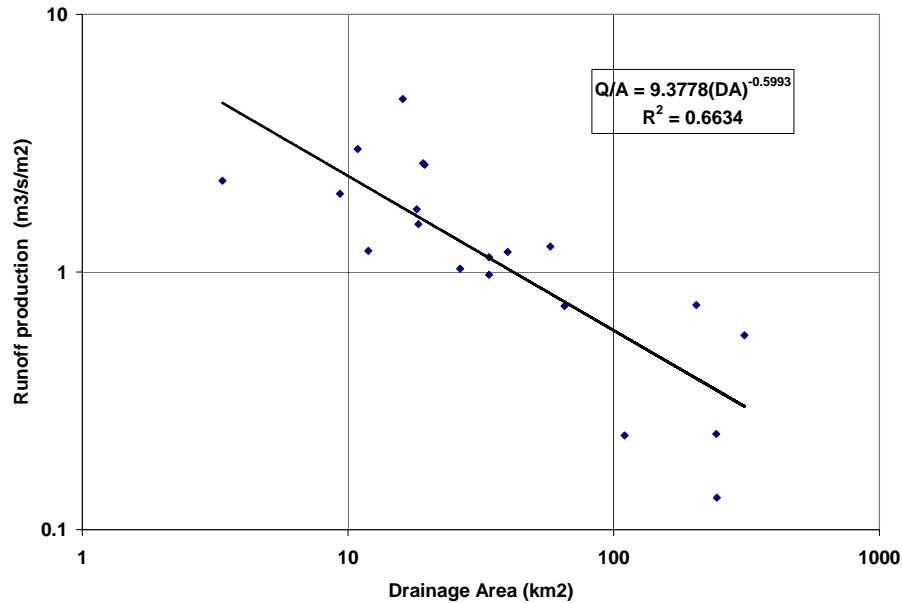
Fig. 6. Runoff production – drainage area relationship for the Yazoo River Basin for the streams CEM Types IV and V.
