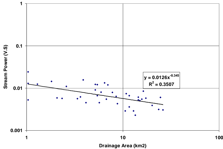
Fig. 9. Unit stream power – drainage area relationship for the Yazoo River Basin for the stream CEM Types II and III.
