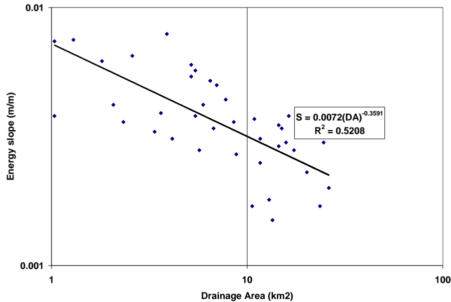
Fig. 5. Channel longitudinal slope – drainage area relationship for the Yazoo River Basin for the stream CEM Types II and III.
