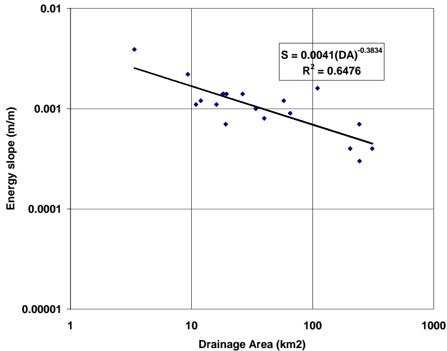
Fig. 4. Channel longitudinal slope – drainage area relationship for the Yazoo River Basin for the streams CEM Types IV and V.
