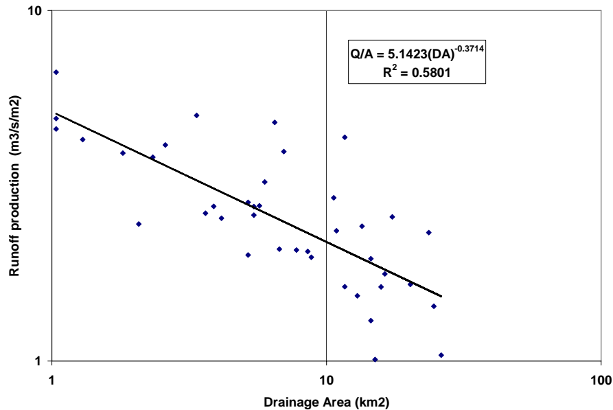
Fig. 7. Runoff production – drainage area relationship for the Yazoo River Basin for the stream CEM Types II and III.
