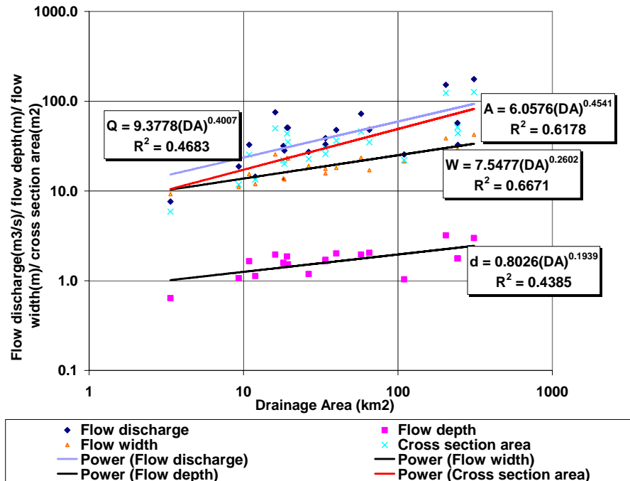
Fig. 2. Channel geometry relationships for the Yazoo River Basin for the streams CEM Types IV and V.
