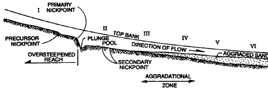
Fig. 1. Incised Channel Evolution Sequence (after Schumm et al., 1984).
