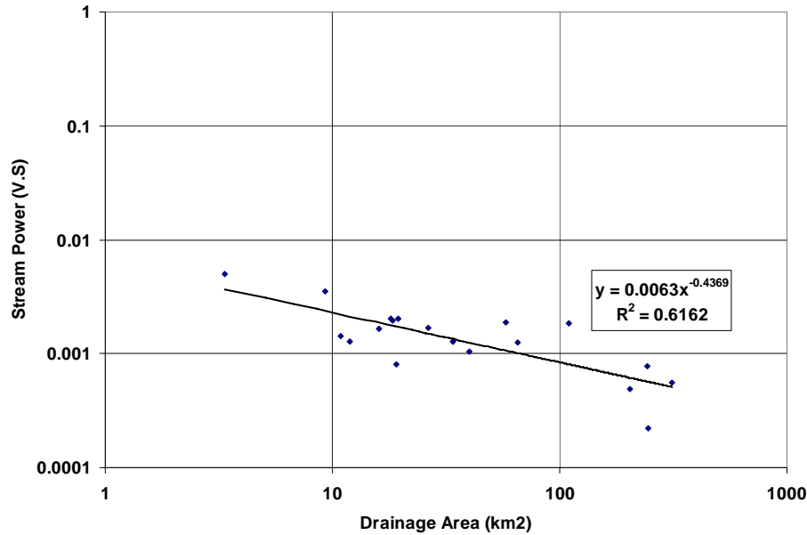
Fig. 8. Unit stream power – drainage area relationship for the Yazoo River Basin for the streams CEM Types IV and V.
