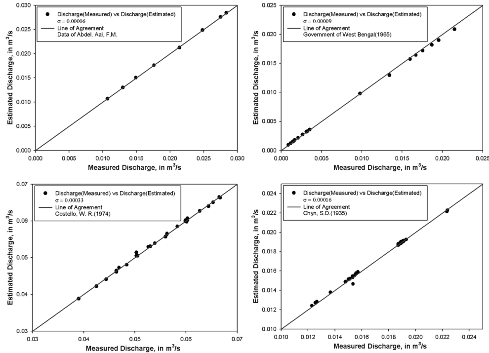
Fig. 4. Analysis results by using proposed mean velocity equation in the lab. channels.
