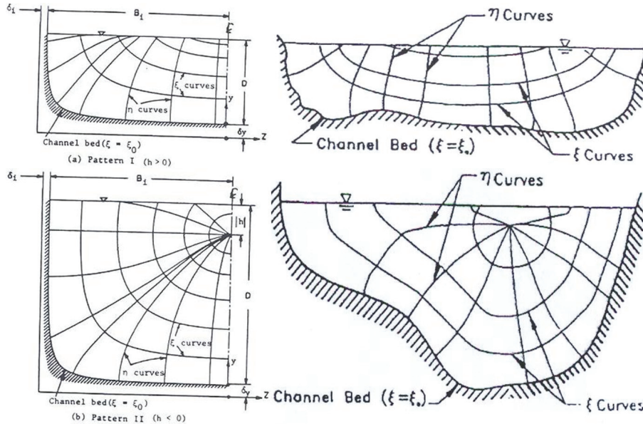
Fig. 1. \xi - \eta coordinates in open-channel sections (Chiu, 1988, 1989).
