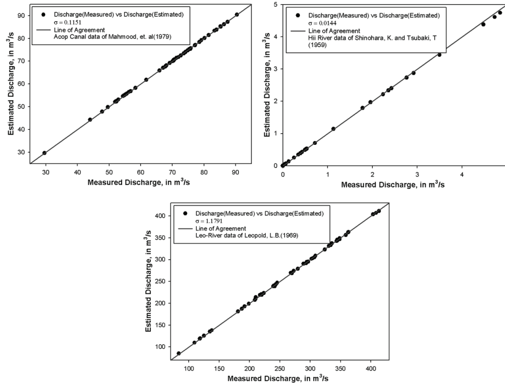
Fig. 5. Analysis results by using proposed mean velocity equation in the natural open channels.
