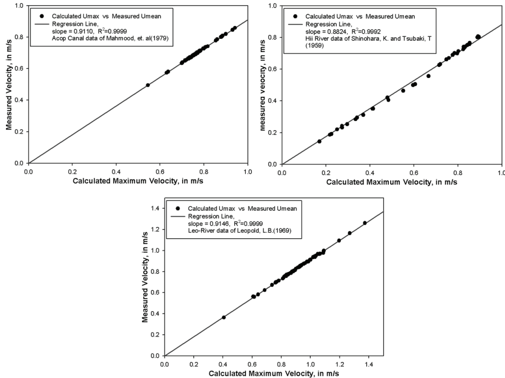
Fig. 3. The relationship between measured mean velocity and calculated maximum velocity in the natural open channels.
