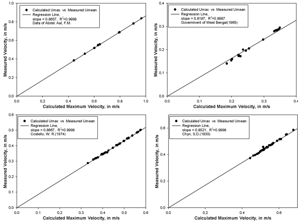
Fig. 2. The relationship between measured mean velocity and calculated maximum velocity in the lab. channels.
