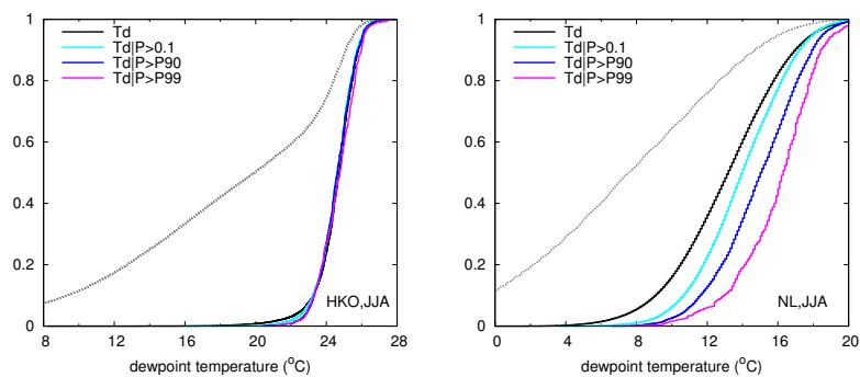
Fig. 3. Cumulative density function (CDF) of the dew point temperature for summer (JJA). Distributions of the dew point temperature are plotted for all hours, for hours with precipitation, and for hours with precipitation exceeding the 90th and 99th percentile of hourly precipitation. As in Fig. 2 dew point temperatures are taken 4 h before the precipitation event. The grey stippled line gives the CDF of all hours for the whole year.
