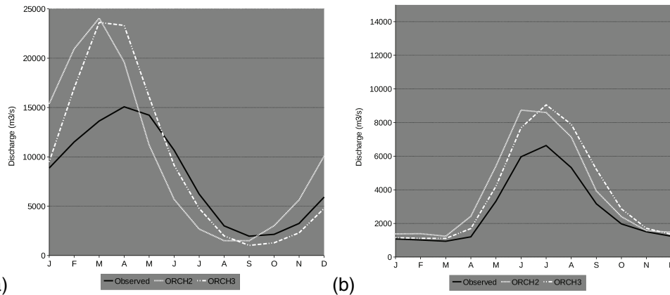
Fig. 15. Mean monthly seasonal discharge ( \text{m}^3 \text{s}^{-1} ) at (a) GMIR and (b) CARA for simulation ORCH3 compared to ORCH2 and observations, over the mean time period 1980–2000.
