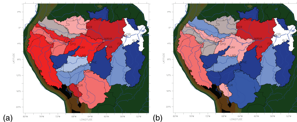
Fig. 9. Mean relative error of Q_{\text{mean}} (%) between simulations ((a) ORCH1, (b) ORCH2) and observation over the time period 1980–2000. The color indicates the sign of the error: red is negative error, blue is positive error and grey is very low error. The error is represented for the different stations (colored circles) and their associated sub-basins (same color than the corresponding station). Five residual basins are also represented: SPO*, MANA*, OBI*, PVE* and FVA*. Q_{\text{mean}} of each residual basin is the difference between the downstream and the upstream station(s) Q_{\text{mean}} . Thus, the color of the residual basin can be different from the color of the downstream station. For topographic scale, see Fig. 2.
