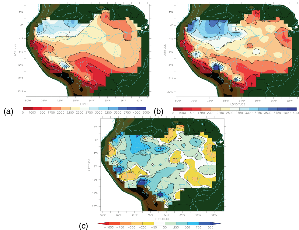
Fig. 3. Precipitation ( \text{mm yr}^{-1} ) over the Amazon River basin from (a) NCC and (b) HYBAM. (c) Differences between (b) and (a). For topographic scale, see Fig. 2.
