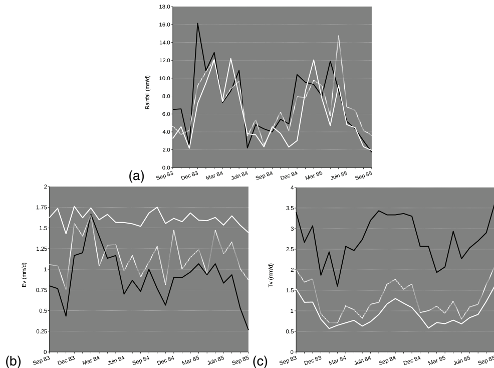
Fig. 8. Comparison of times series of (a) precipitation ( P ), (b) evaporation of water over the leaves ( E_v ) and (c) transpiration ( T_v ) (all in \text{mm d}^{-1} ) between the two simulations (ORCH1 and ORCH2) and estimates from Shuttleworth (1988) near Manaus (Ducke Reserve), over the period September 1983–September 1985.
