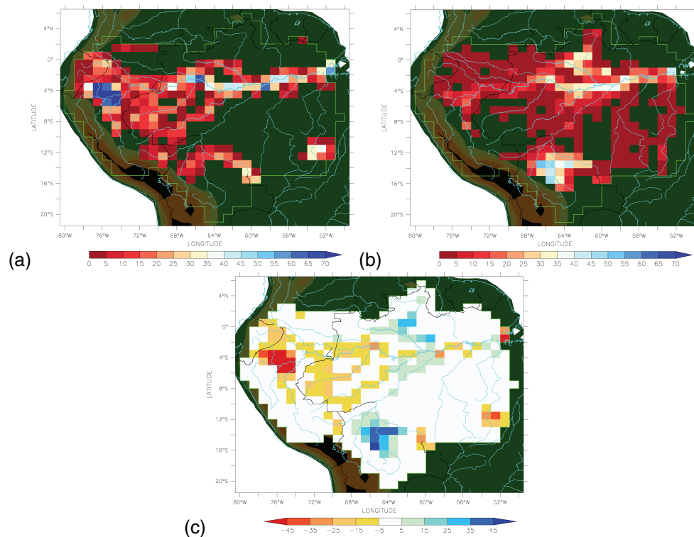
Fig. 5. Fraction of swamps within the mesh (% of the mesh area) over the Amazon River basin from (a) GLWD and (b) PRIMA. (c) Differences between (b) and (a) . Dark green and brown colors indicate the topography of the region. For topographic scale, see Fig. 2.
