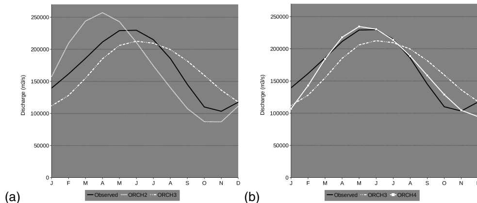
Fig. 14. Mean monthly seasonal discharge (m 3 s -1 ) at OBI for simulation ORCH3 compared to (a) ORCH2 and (b) ORCH4. Comparison with observations is shown over the mean time period 1980–2000.
