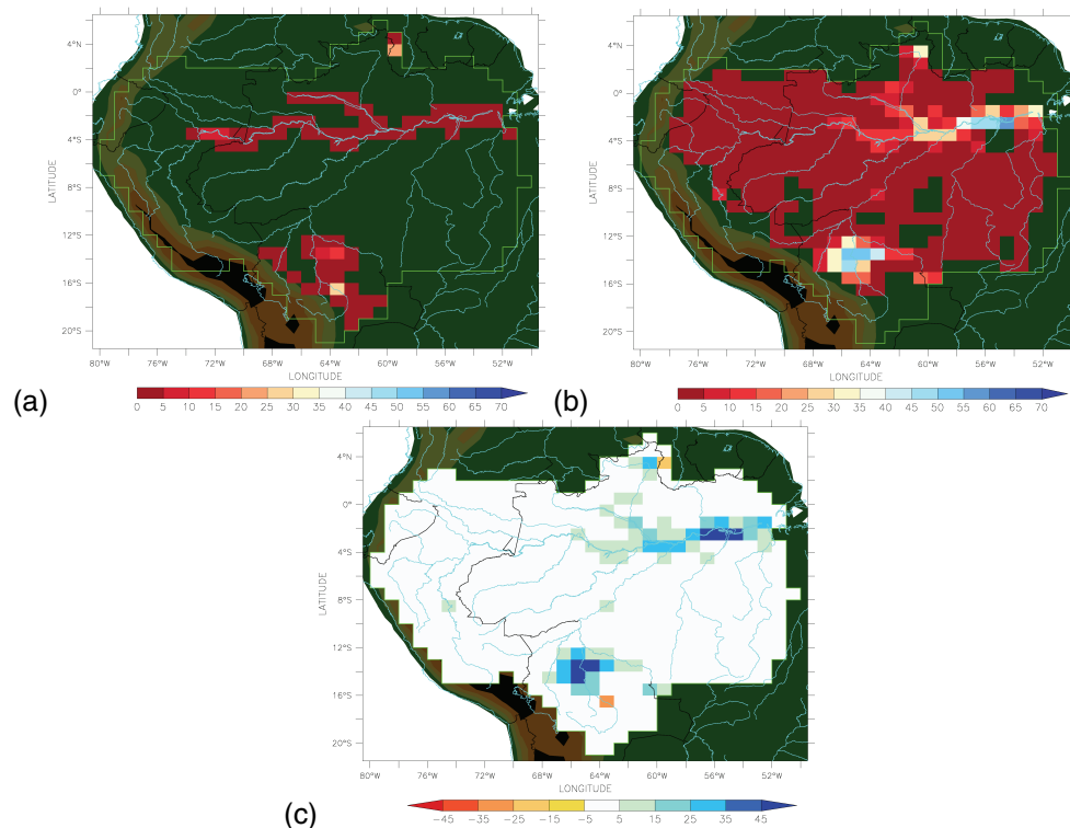
Fig. 4. Fraction of floodplains within the mesh (% of the mesh area) over the Amazon River basin from (a) GLWD and (b) PRIMA. (c) Differences between (b) and (a) . Dark green and brown colors indicate the topography of the region. For topographic scale, see Fig. 2.
