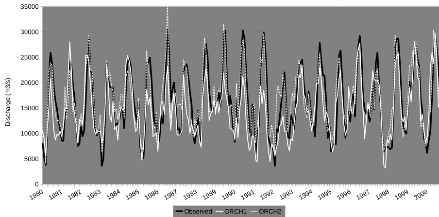
Fig. 12. Interannual variation of monthly discharge ( \text{m}^3 \text{s}^{-1} ) at SER for simulations ORCH1 and ORCH2 compared to observations, over the time period 1980–2000.
