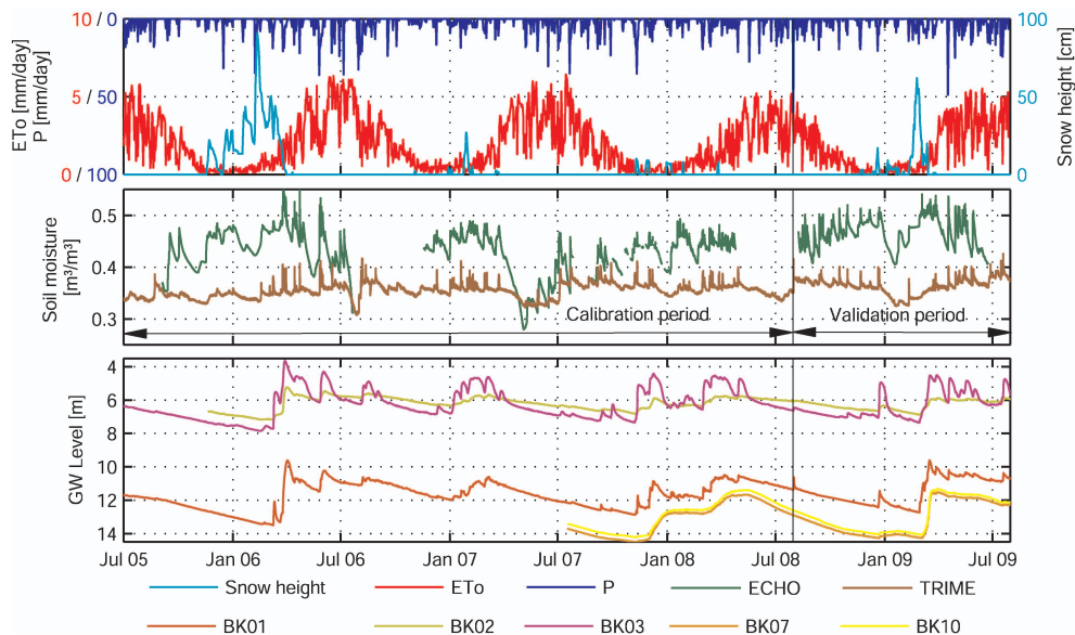
Fig. 2. Time series of input and calibration data. Time series of daily precipitation ( P ), daily reference evapotranspiration ( ET_o ) and snow height (top). Time series of soil moisture (middle) and groundwater data (bottom).
