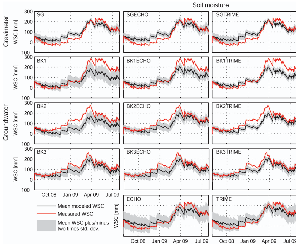
Fig. 5. Measured versus modelled WSC for the validation period of July 2008 to July 2009.
