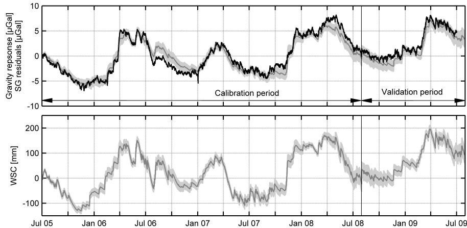
Fig. 7. SG residuals (black line) and modelled gravity response (grey band) (top). Modelled water storage change (bottom). The model was calibrated against the SG residuals for the period of 1 July 2005 to 30 July 2008.
