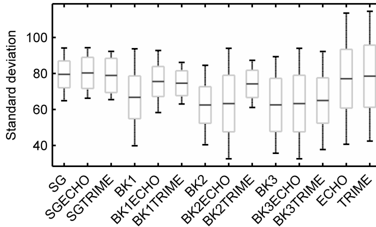
Fig. 4. Performance of the different models for the calibration period. The median of the box plot is a measure of the signal amplitude (the standard deviation of the mean signal). The box and whiskers represent the scattering of the standard deviation of the behavioural model runs computed at each time step. (The standard deviation of the mean signal was added to the standard deviation of the behavioural model runs at each time step).
