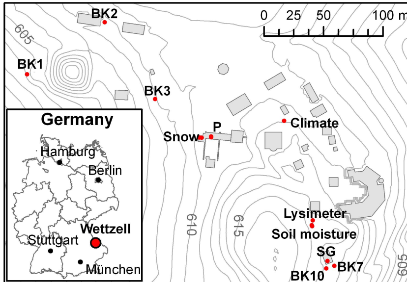
Fig. 1. Study area with the different hydrological sensors and the topography represented by contour lines (distance 1 m). Location of Wetzell in Germany and some major cities are displayed in the inset map.
