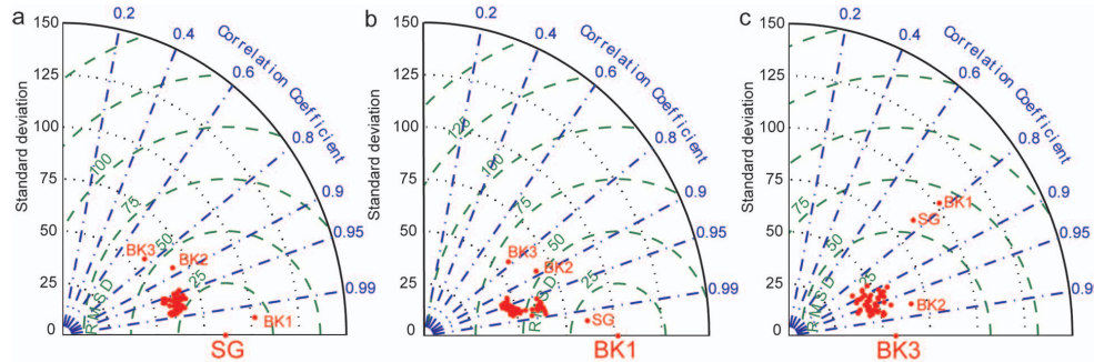
Fig. 6. Taylor diagrams (Taylor, 2001) comparing measured and modelled WSC for the models SG (a), BK1 (b) and BK3 (c). Each figure also contains the measured WSC for the other sites.
