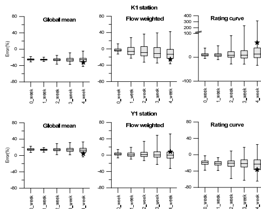
Figure 1. The possible errors versus different sampling interval and flux calculation methods
