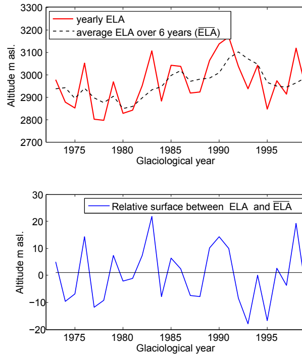
Fig.1: top: yearly ELA and \overline{ELA} over 6 years for the Rhone glacier; \overline{ELA} is assumed to approximate the elevation of the firn line; bottom: amount of glacier surface (in %) that corresponds to the altitude difference of ELA and \overline{ELA} ; this surface is positive if ELA > \overline{ELA} , it is negative if ELA < \overline{ELA} ; positive values indicate exposed firn.
