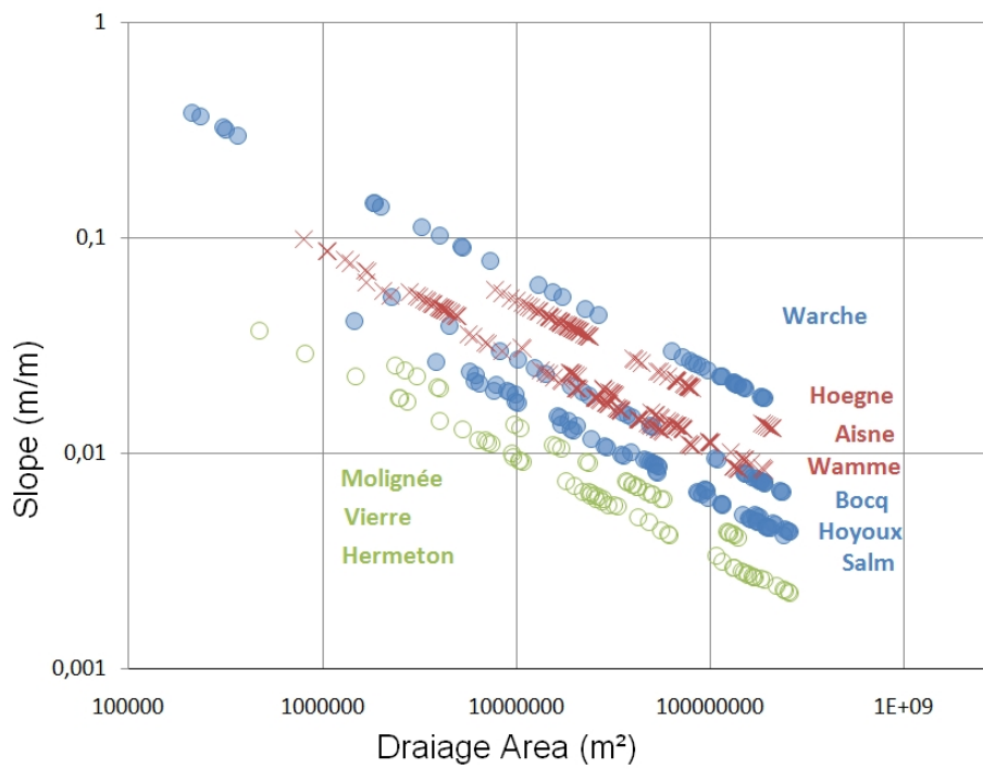
Fig. 2. Annex2 : Ksn distribution in AxS space
