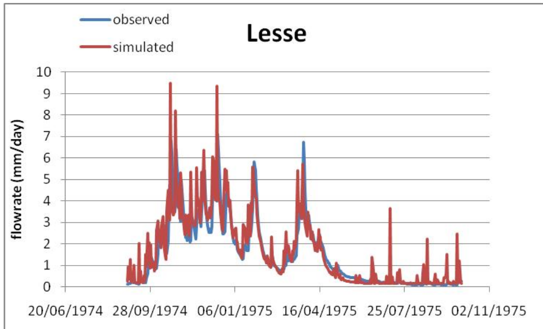
Fig. 2. validation periods for the Lesse
