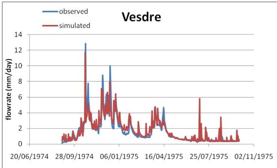
Fig. 1. validation periods for the Vesdre
