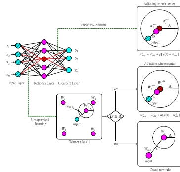
Figure 1 The architecture of CFNN with training procedure.
