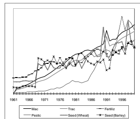
Figure 2. Evolution of management indicators: farm equipment power (Mac), tractors (Trac), nitrogen fertilizer (Fertiz), pesticide consumption (Pestic), or seeds improvement (Seed). Source: Quiroga, Iglesias, 2010.
