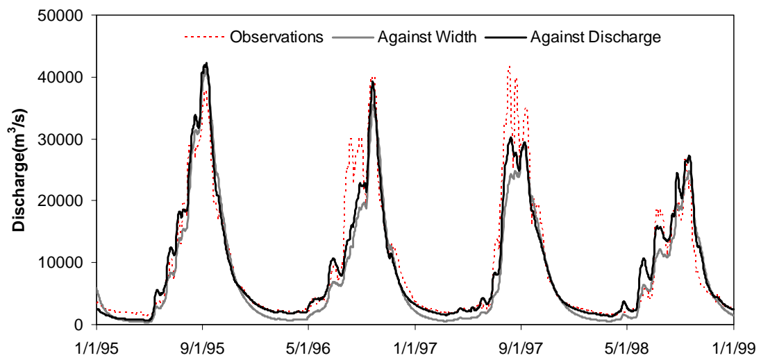
Discharge time series at Pakse from observations, mean simulation of behavioral parameter sets by calibration against satellite observations of river width, and best simulation by calibration against observed discharge data.
