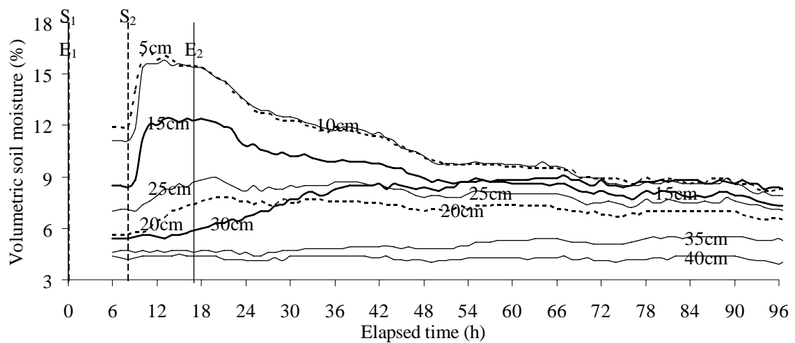
Fig. 6. The wetting front advance from 14:00 LT of 28 August to 14:00 LT of 1 September. Vertical lines of paired S and E represent the start and end of individual rainfall respectively.
