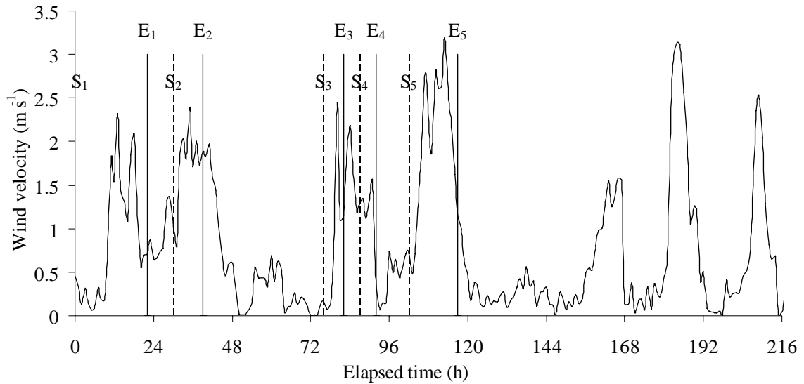
The wind velocity during the period from 0:00 LT of 22 September to 0:00 LT of 1 October. The vertical lines are the same as in Fig. 7.
