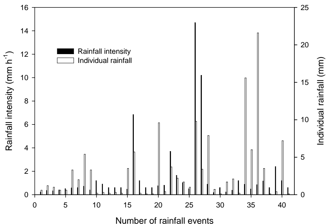
Fig. 2. Rainfall intensity and individual rainfall of the total 41 rainfall events in the year 2008 at the experimental site.
