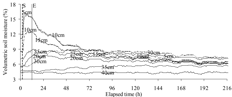
Fig. 6. The wetting front advance from 20:00 LT of 28 August to 20:00 LT of 7 September (S) represents the start of rainfall, (E) the end of rainfall.
