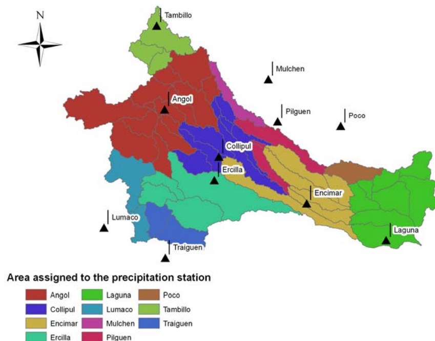
Figure R-1. Subbasins and the location of the corresponding meteorological station
