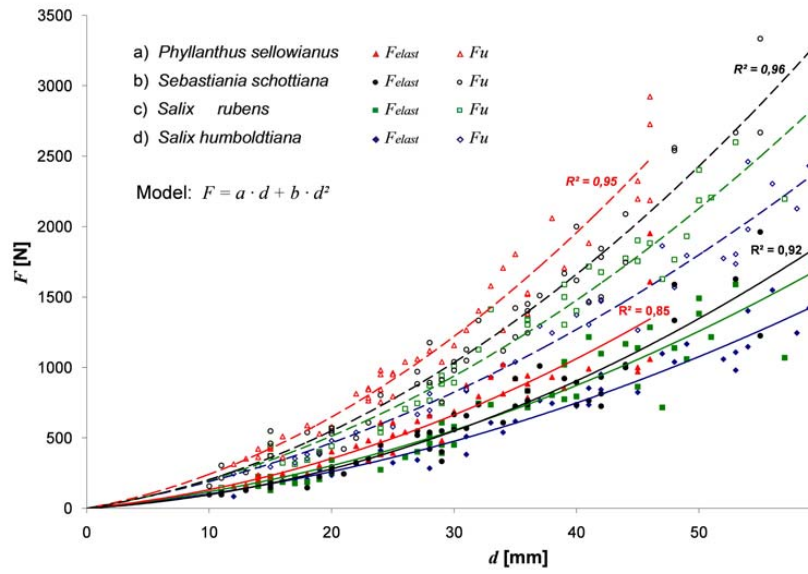
Fig. 3: Relationship between diameter ( d ) and load ( F ). Solid line: F_{elast} at the pr dashed line: F_u at the point of rupture.
