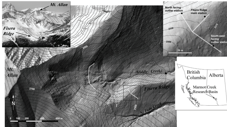
Fig. 1. Shaded topographic map of Fisera Ridge and the Upper Middle Creek Basin (hatched area) within the Marmot Creek Research Basin, Alberta. Snow survey transects in 2008 are represented by the dashed lines and location of the detailed Fisera Ridge inset map is indicated. Other insets include an aerial photograph of the basin and a map showing the location of Marmot Creek within Western Canada.
