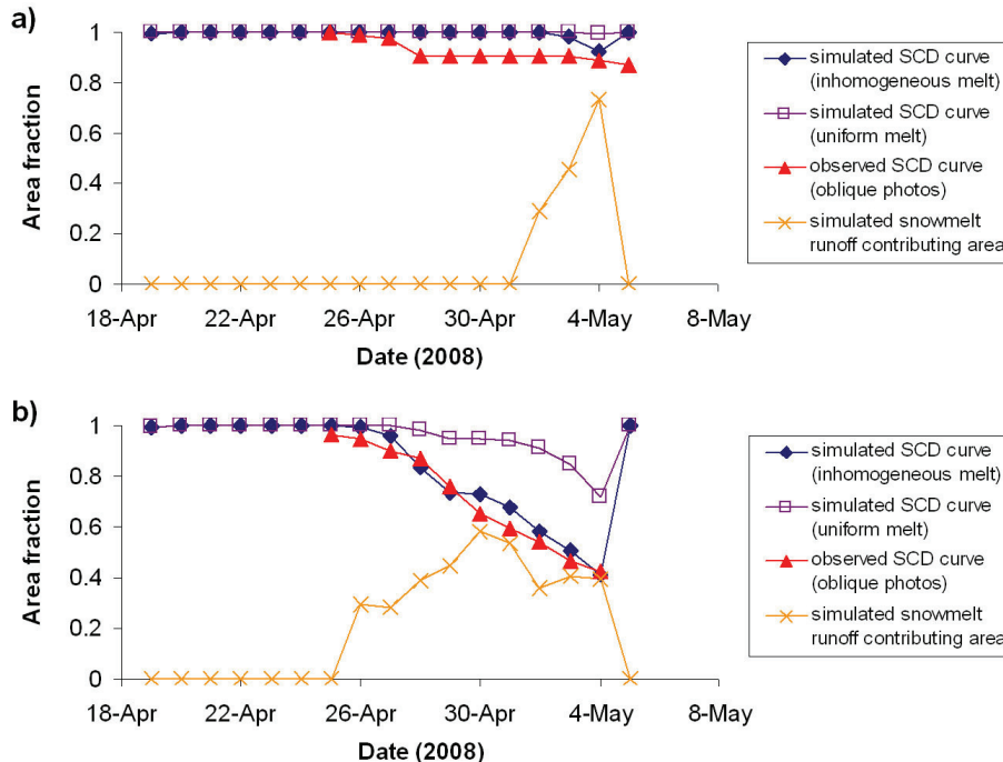
Fig. 4. Simulated vs. observed SCD curves and the SRCA during the early melt period within the Mt. Allan cirque in 2008: (a) North-facing slope unit; (b) South-facing slope unit. SCD curves were derived based on uniform slope-based melt rates and melt rates obtained from computations based on different initial SWE values (inhomogeneous melt). Observed SCD curves were derived from the orthogonally corrected photographs of the cirque.
