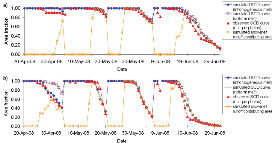
Fig. 5. Simulated vs. observed SCD curves and the SRCA over the entire spring period within the Mt. Allan cirque in 2008: (a) North-facing slope unit; (b) South-facing slope unit.
