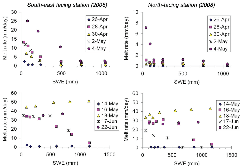
Fig. 3. Plots of SWE vs. simulated melt rates at different times in the melt period of 2008 on two opposite slopes over Fisera Ridge.
