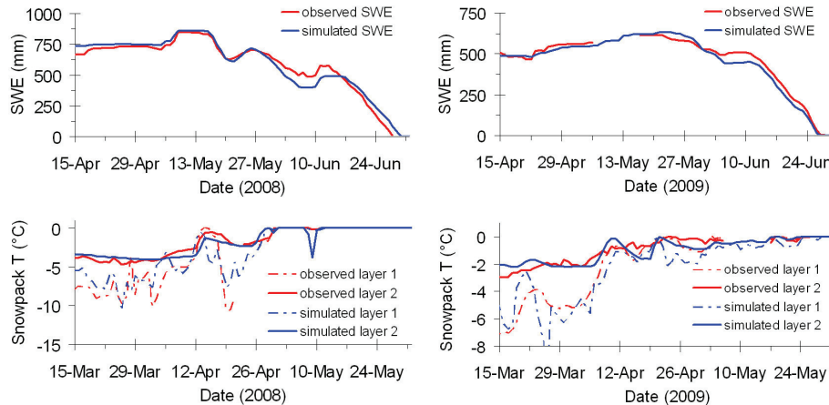
Fig. 2. Comparison of simulated and observed SWE and internal snowpack temperature at the south-east facing outlier site on Fisera Ridge during the melt period in 2008 (calibration) and 2009 (validation).
