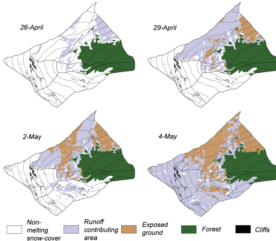
Fig. 7. Spatial snow-cover and SRCA patterns over the Upper Middle Creek Basin (showing the four different slope-based HRUs) in the early snowmelt period of 2008. Patterns were mapped based on the spatial distribution of snow depth and SWE derived from the repeat LiDAR data. Snow melt patterns were not simulated in the densely forested or cliff areas.
