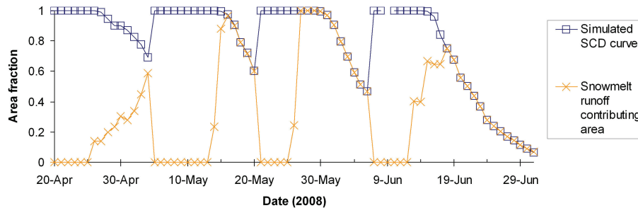
Fig. 6. Simulated basin-scale SCD curve and SRCA over the Upper Middle Creek Basin for the spring period of 2008.
