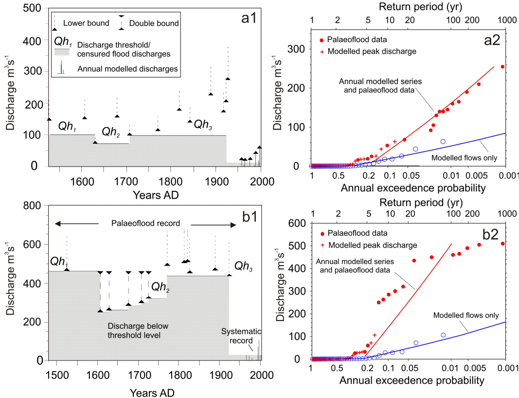
Fig. 8. Palaeoflood and modelled discharges at Rooifontein ( a1 ) and Messelpad ( b1 ). The horizontal shaded areas represent the discharge threshold values ( Q_h ) used in the flood frequency analysis. Two component extreme value distributions fitted to annual series of modelled discharges and palaeoflood information (censored data) for Rooifontein ( a2 ) and Messelpad ( b2 ).
