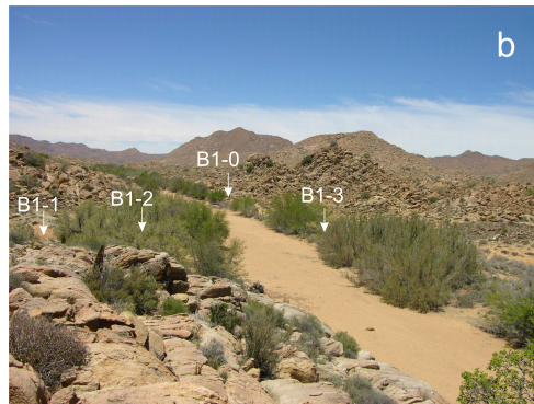
Fig. 6. Rooifontein study reach: (a) Longitudinal profile of the stream channel bed and water surface profiles obtained from HEC-RAS modelling for the highest palaeoflood deposits ( 310 \text{ m}^3 \text{ s}^{-1} ) and for a reference discharge of 100 \text{ m}^3 \text{ s}^{-1} . Stratigraphic profiles are represented as vertical bars, with colours sketching flood sediments of different age. (b) General upstream view of the Rooifontein reach and location of two four stratigraphic profiles B1-0, B1-1, B1-2 and B1-3.
