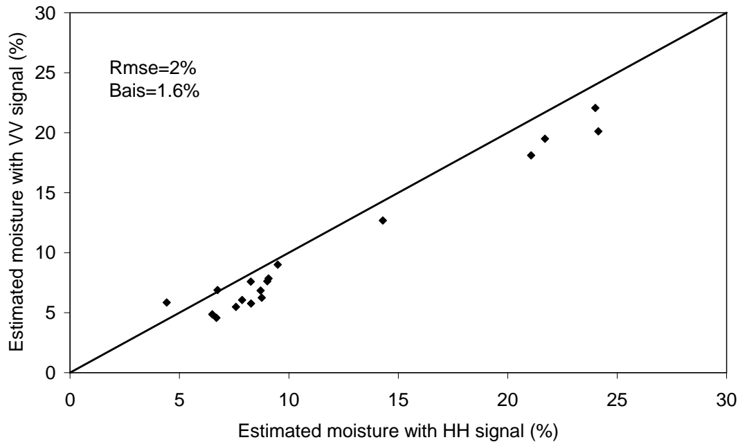
Fig. 8. Inter-comparison between HH and VV radar signal moisture estimations.
