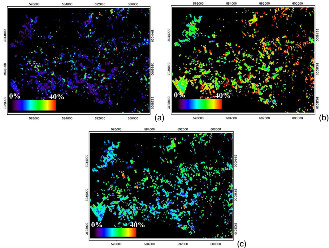
Fig. 15. Example of moisture mapping over wheat fields on three different dates: (a) 24 December 2008, (b) 16 January 2009, (c) 7 March 2009.
