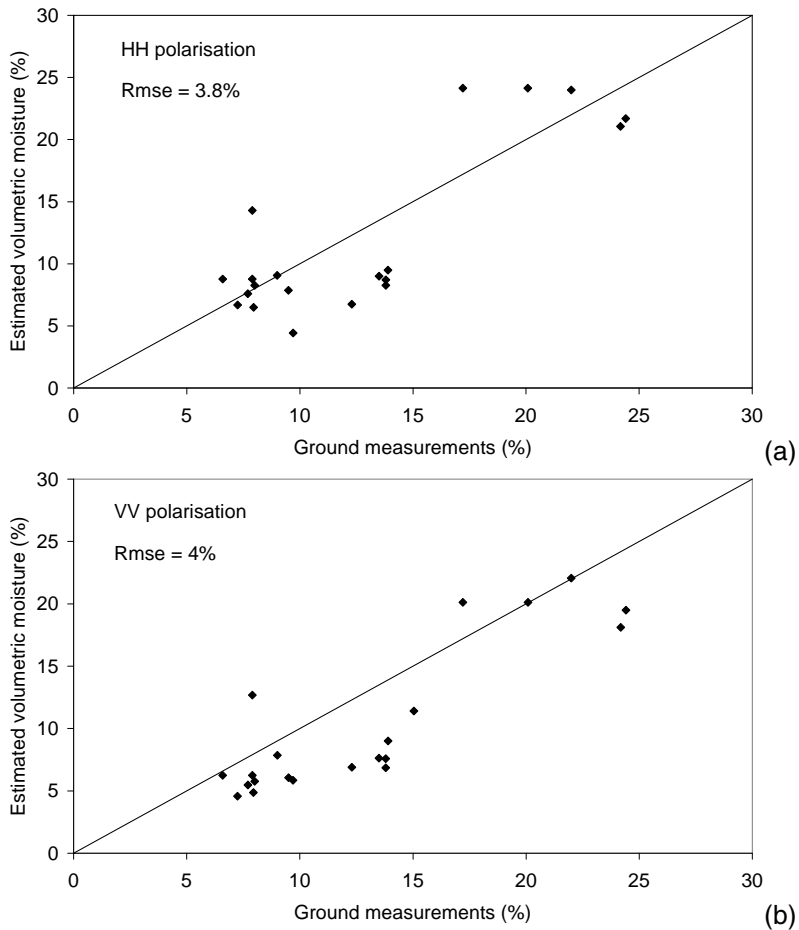
Fig. 7. Soil moisture estimations from ASAR/ENVISAT data, expressed as a function of the soil moisture derived from ground-truth measurements, for fields in the “olive tree” class of land use, (a) HH polarisation, (b) VV polarisation.
