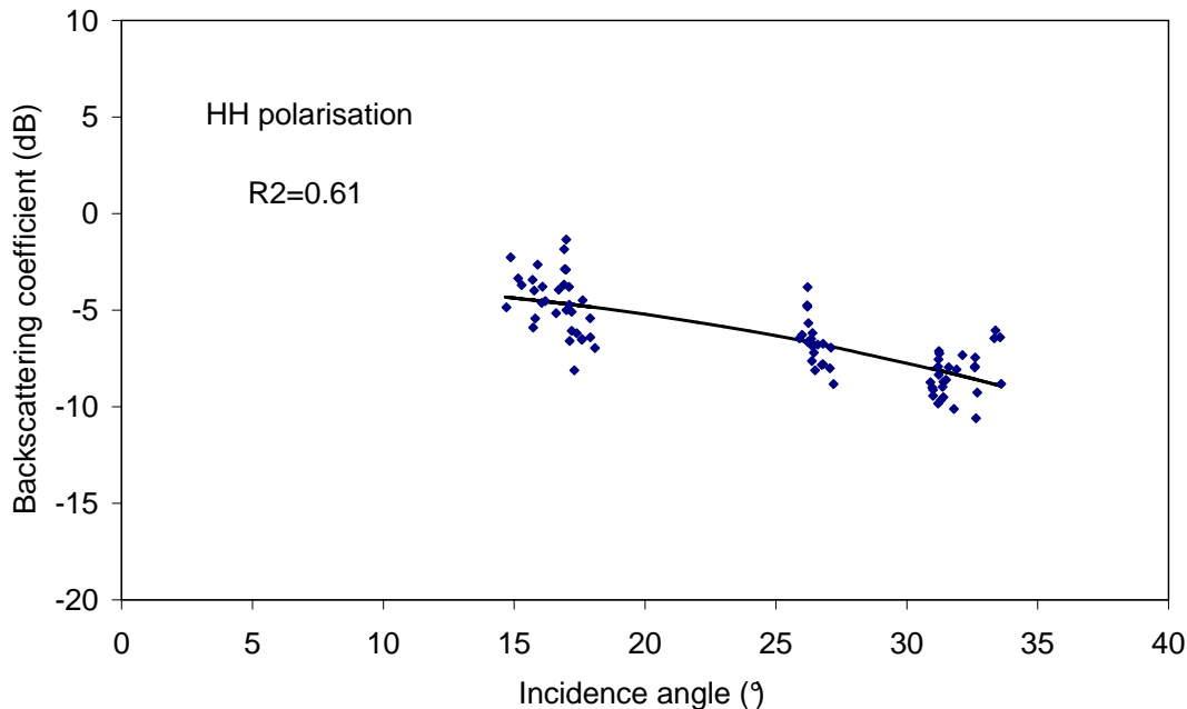
Fig. 11. Illustration of ASAR HH polarisation data over bare soils after wheat sowing, as a function of incidence angle.
