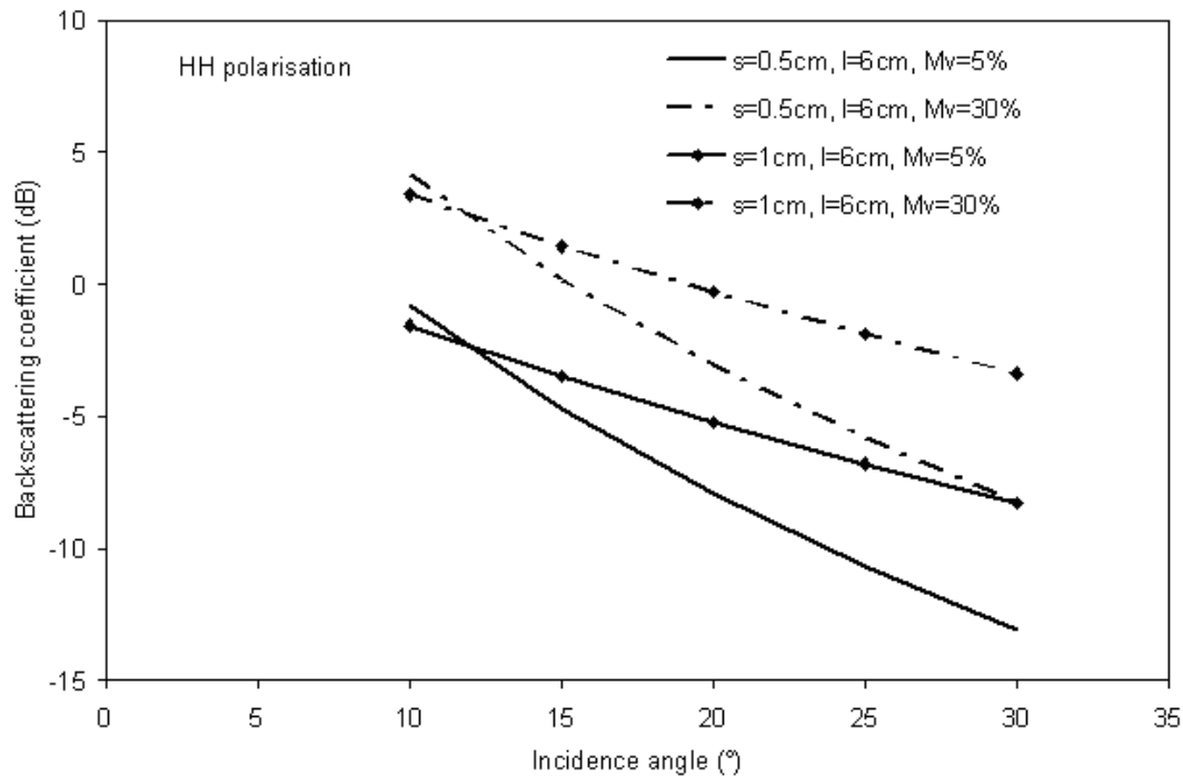
Fig. 10. IEM simulations of backscattering coefficient variation as a function of incidence angle, for different moisture and roughness values.
