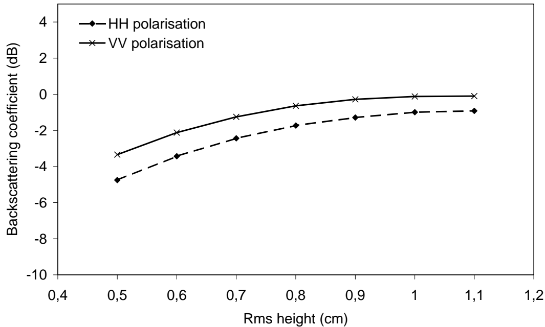
Fig. 5. Illustration of backscattering coefficient IEM simulations function of surface roughness (rms height) for HH and VV polarisations.
