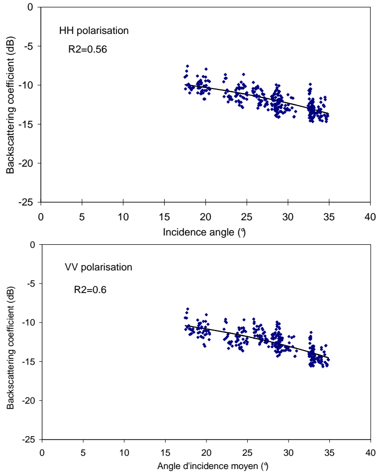
Fig. 4. Angular dependence of backscattered ASAR signals for HH and VV polarizations. The ASAR images were acquired in the IS1, IS2 and IS3 modes.
