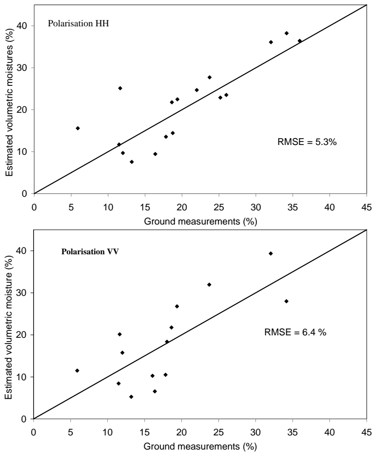
Fig. 13. Soil moisture estimations from ASAR/ENVISAT data, versus soil moisture derived from ground truth measurements, for different test wheat fields.
