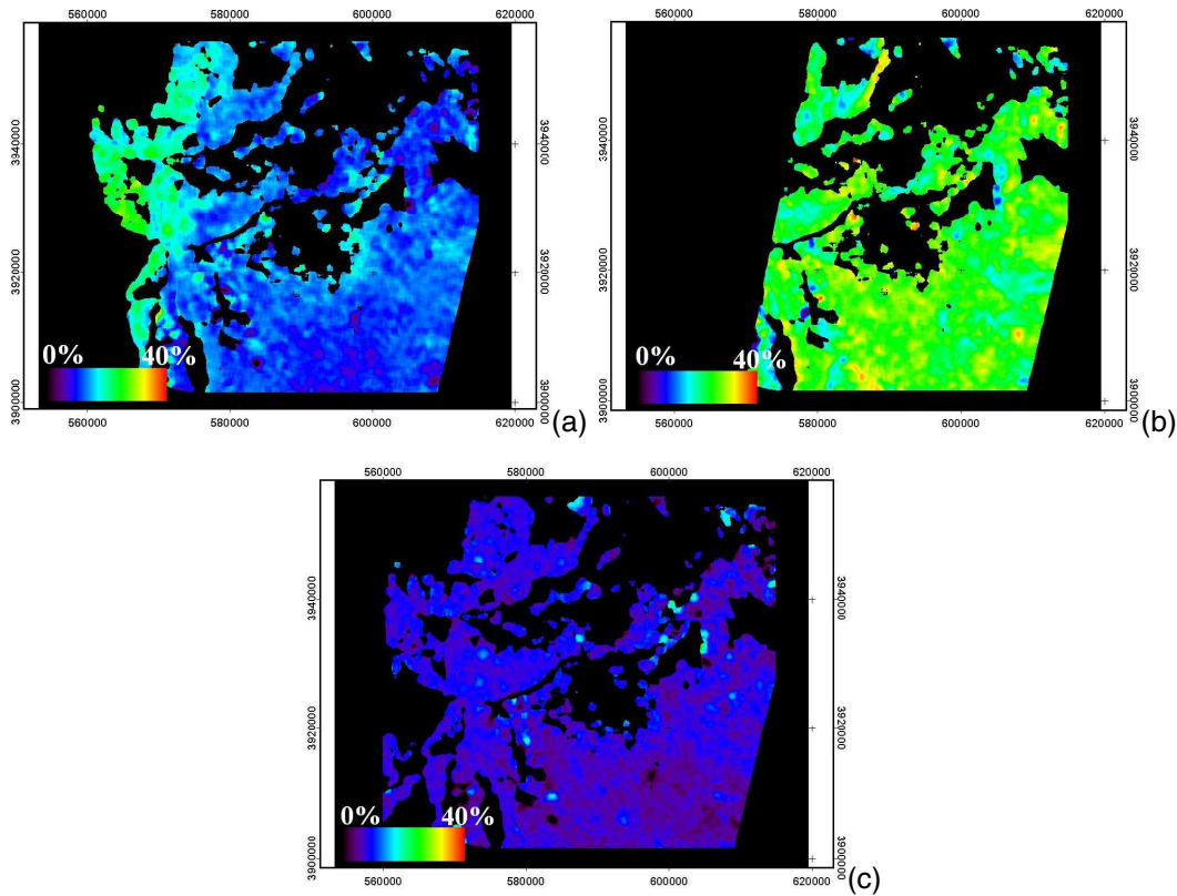
Fig. 9. Illustration of moisture mapping for an area containing fields in the “olive tree” class of land use, (a) 11 April 2009, (b) 12 April 2009, (c) 9 December 2009.
