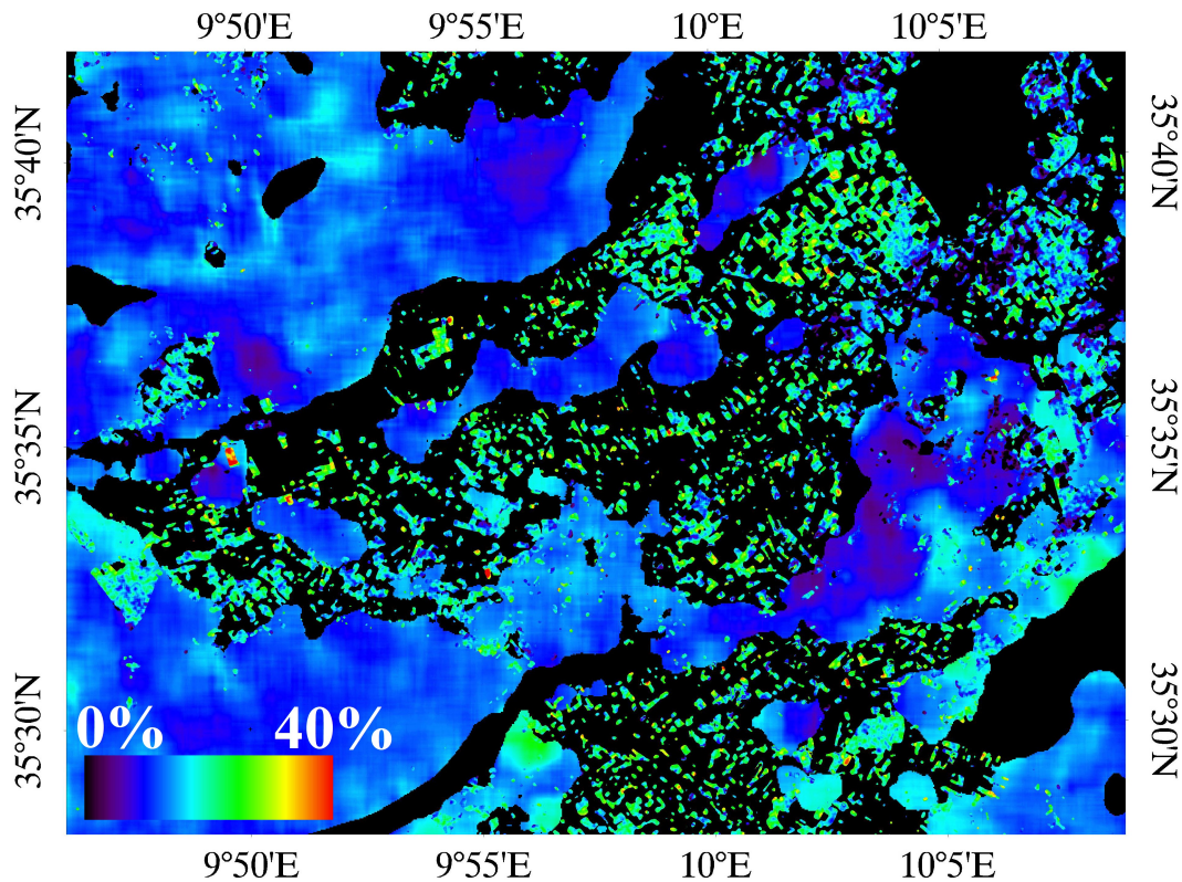
Fig. 16. Example of moisture mapping, showing soil moisture estimations for fields in the “olive tree” and “wheat” classes of land use on 7 March 2009.
