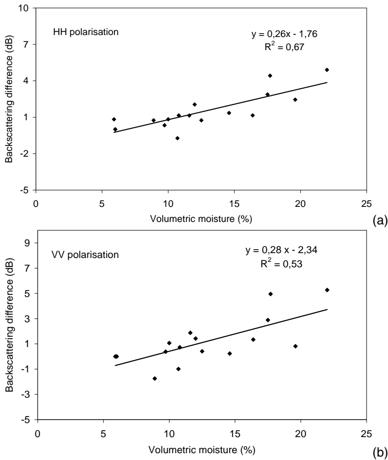
Fig. 6. Processed ASAR/ENVISAT signals (in decibels) versus measured volumetric moisture over olive tree fields, (a) HH polarization, (b) VV polarization.
