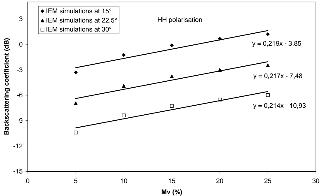
Fig. 12. IEM simulations as a function of soil moisture in HH polarisation, for three incidence angles: 15°, 22.5° and 30°.
