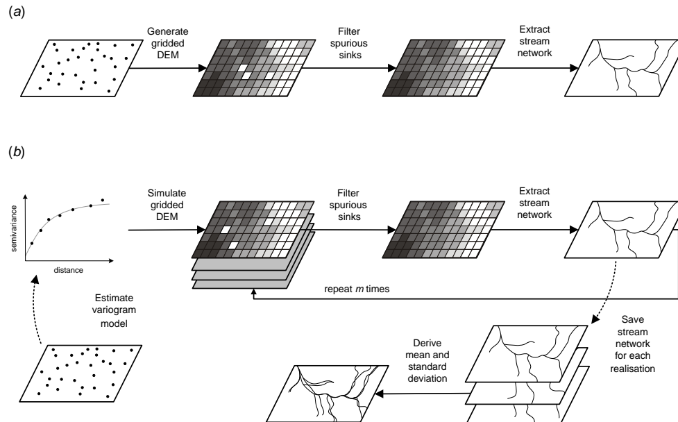
Fig. 1. Workflow scheme for stream extraction from elevation data: (a) assuming that elevations carry no uncertainty; (b) the Monte Carlo error propagation approach with m realizations.
