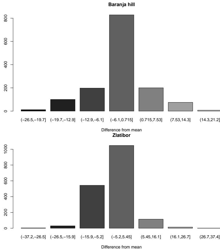
Fig. 7. Bar plots showing relationship between the relative relief (difference from the mean) and cumulative errors. In both cases the highest errors of mapping streams are in areas of low local relief (slightly concave).
