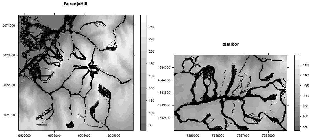
Fig. 5. 100 realizations of stream network overlaid on top of each other: (left) Baranja hill case study; (right) Zlatibor case study.
