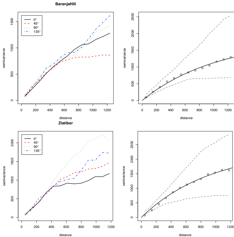
Fig. 4. Variograms fitted for Baranja hill (above) and Zlatibor case studies (below): (left) anisotropy in four directions; (right) isotropic Matérn variogram model fitted using the weighted least squares (WLS) and its confidence bands.
