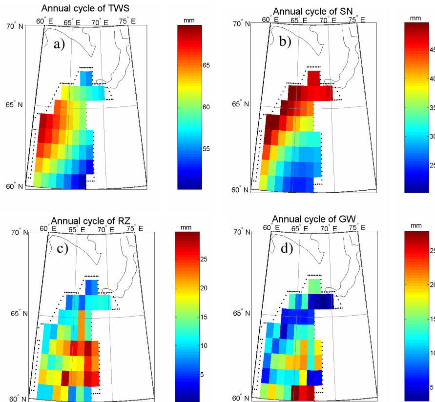
Fig. 8. Amplitude of the annual cycle over 2003–2004: (a) TWS from GRACE, (b) Snow Water Equivalent (SWE) from GRACE, (c) Water in the Root zone from hydrological models, (d) Groundwater and permafrost. Units: mm.
