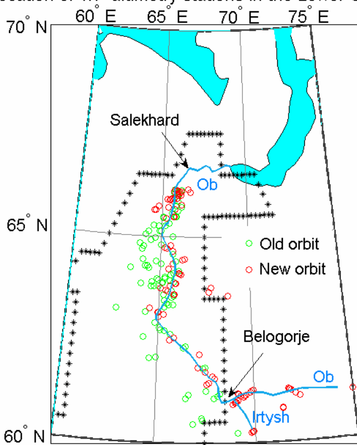
Fig. 1. Map of Lower Ob' basin and locations of the Topex/Poseidon water level stations. The line with stars shows the delineation of the watershed.
