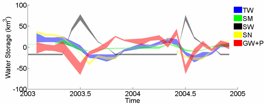
Fig. 7. Monthly variations of TWS volume (blue), surface water volume from T/P radar altimetry and multisatellite inundation dataset (black), soil moisture from hydrological model outputs (green), snow derived from GRACE measurements (yellow), sum of groundwater and permafrost by difference between TWS and the other compartments (red). Units: \text{km}^3 .
