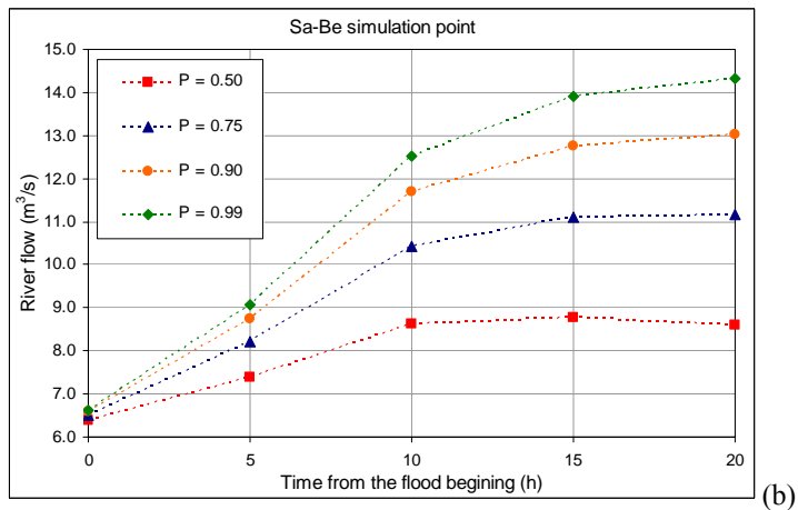
Fig. 8. Temporal evolution of streamflow for storm events during summer period. Each curve is related to a storm non-exceedance probability value. Simulation points are Be3 (a) and Sa-Be (b).
