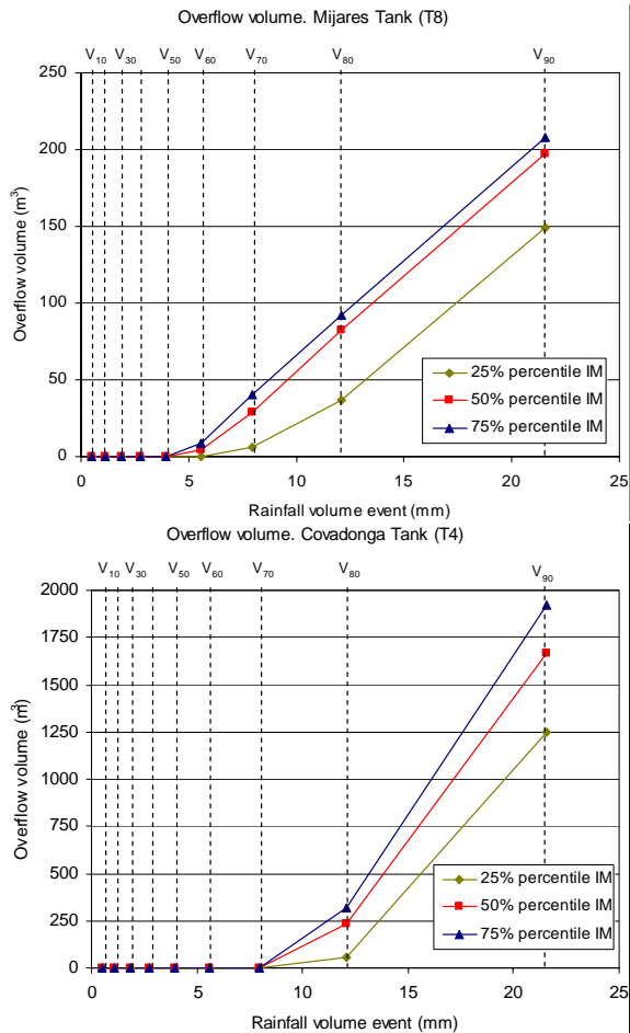
Fig. 5. Storage system diagnosis: spilled volume.
