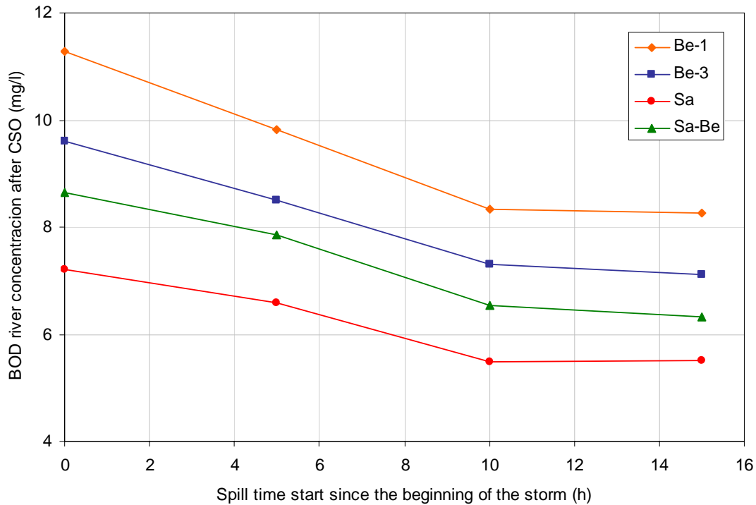
Fig. 10. BOD concentration in the river after CSO for the non-exceedance storm probability P=0.75 .
