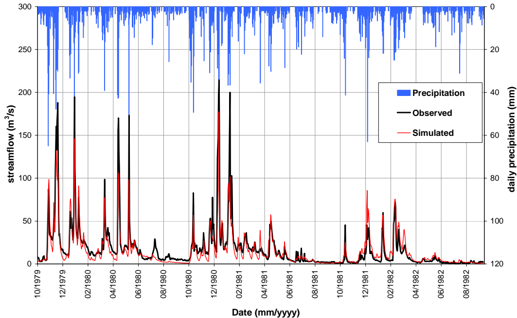
Fig. 6. Daily precipitations and streamflows observed and simulated with TETIS model at Be3 point during the calibration period.
