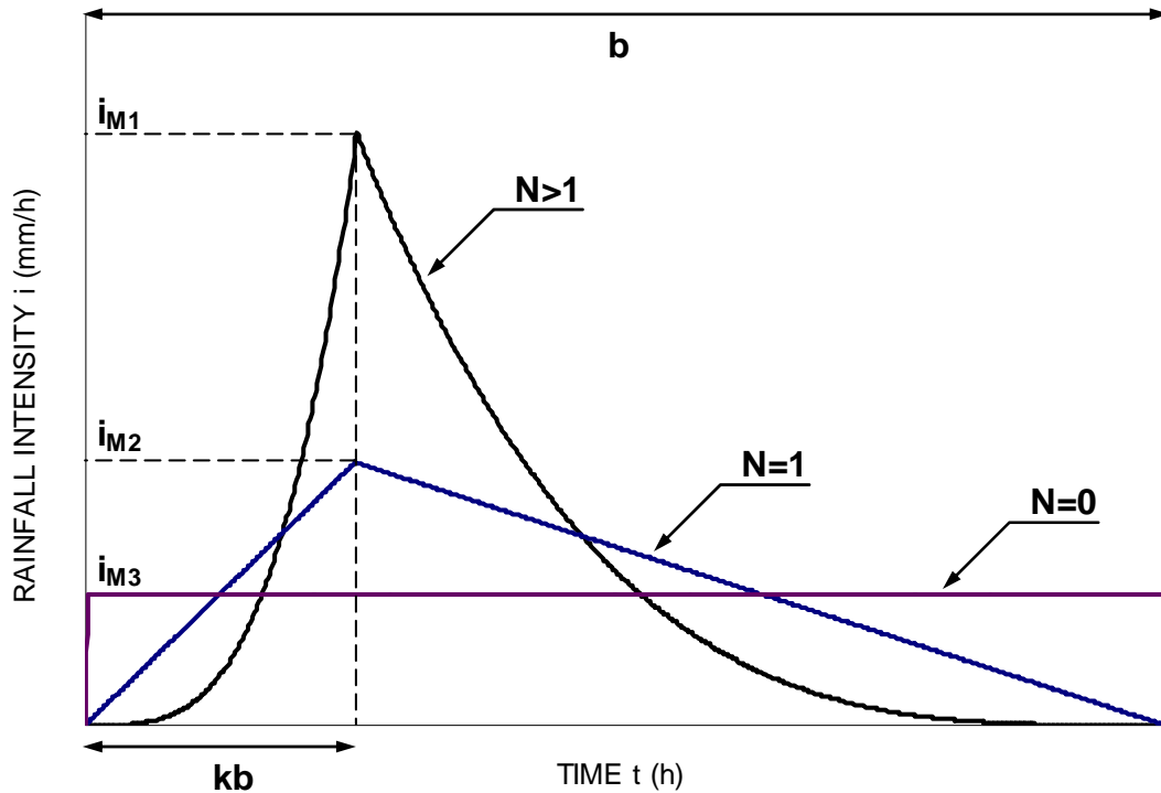
Fig. 3. Synthetic storm shape depending on N -parameter.
