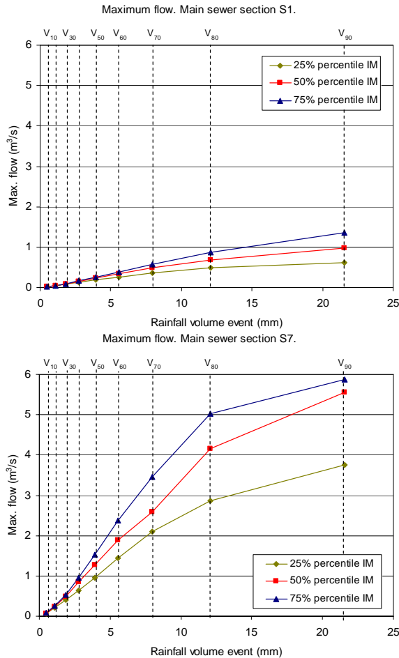
Fig. 4. Interception system diagnosis: maximum sewer flow.
