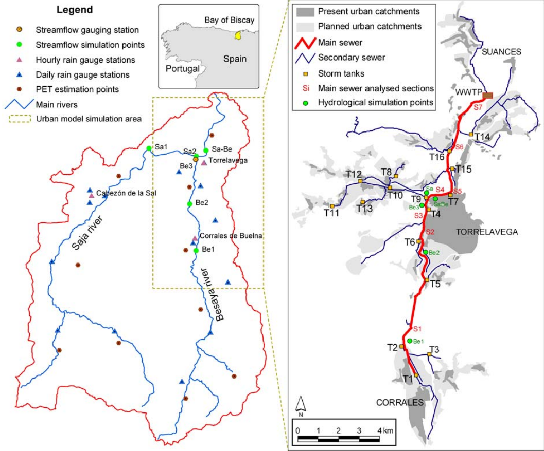
Fig. 1. River basin, main drainage network, rain-gauges, gauging point, PET estimation points and fluvial simulation points. Right: Present urban catchment and future planning, main and secondary sewers, storm tanks and main sewer sections location, and WWTP.
