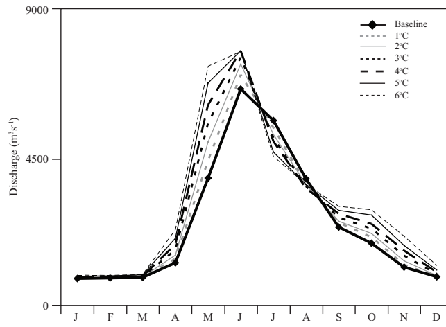
Fig. 8. Comparison of baseline and projected mean monthly river discharge under prescribed increases of 1 to 6°C in global mean air temperature by HadCM3.
