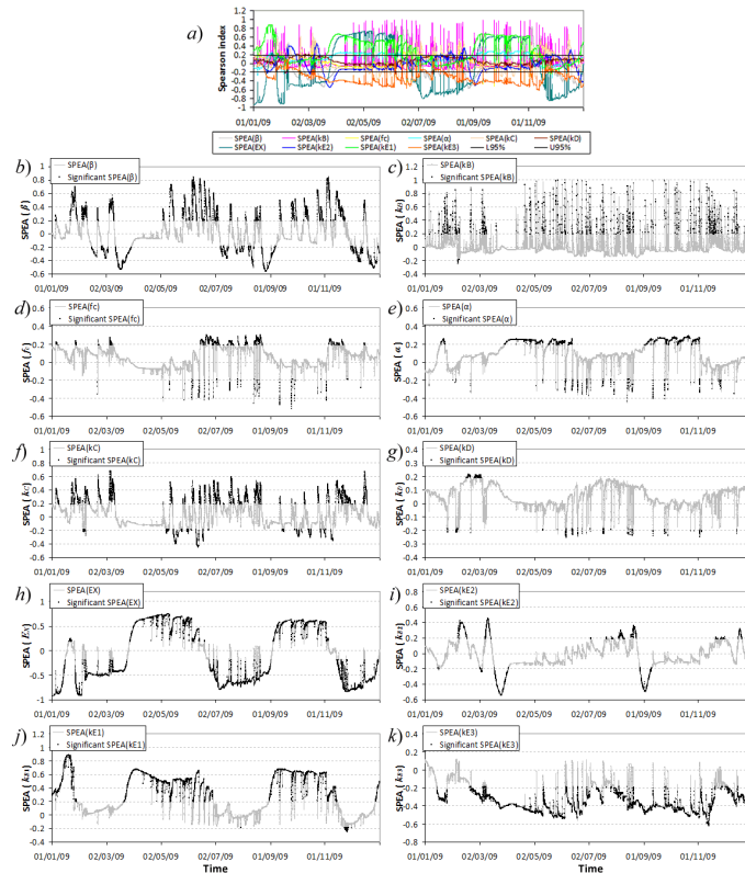
Fig. 10. Spearman indexes between Q and (a) all the parameters: black horizontal lines indicate the 95% confidence interval out of which the Spearman is significant, (b) partition parameter \beta , (c) surface discharge k_B , (d) infiltration rate at field capacity f_c , (e) maximum infiltration \alpha , (f) root-reservoir discharge k_C , (g) non-root discharge k_D , (h) threshold for shallow aquifer E_X , (i) shallow aquifer discharge k_{E2} , (j) deep aquifer discharge k_{E1} and (k) deep percolation discharge k_{E3} . The black dots indicate the time steps for which the Spearman is significant at the 95% confidence level, while grey dots indicate non-significant correlations.
