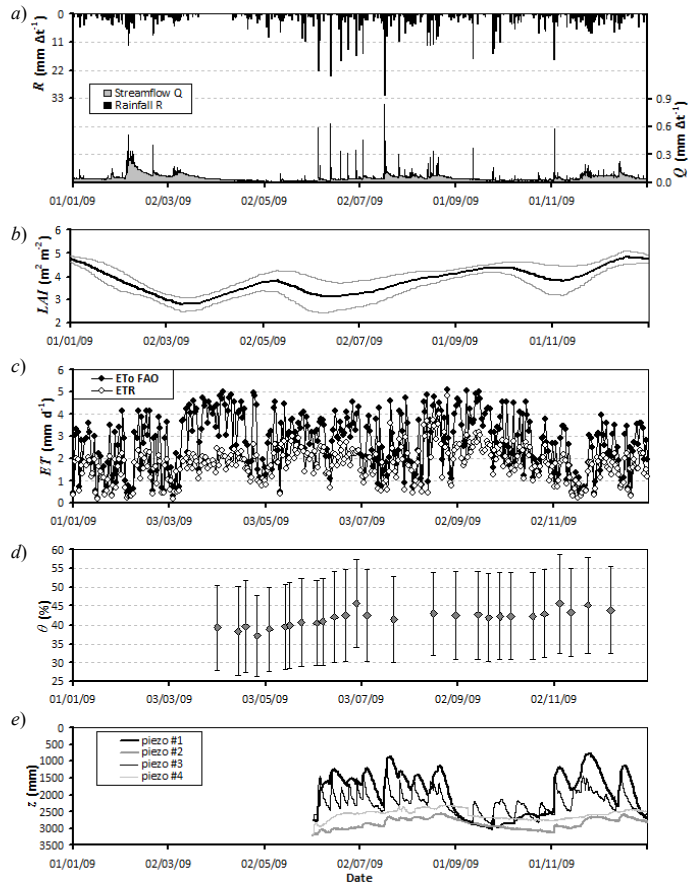
Fig. 5. Measurements in the experimental basin for 2009: (a) rainfall R and streamflow Q , \Delta t=30 min, (b) leaf area index (LAI) within 1 std. dev. confidence bands (grey), (c) reference-potential ( ET_0 ) and measured (ETR) daily evapotranspiration, (d) soil water content \theta with one standard deviation bars and (e) water table level z in the four piezometers throughout the basin.
