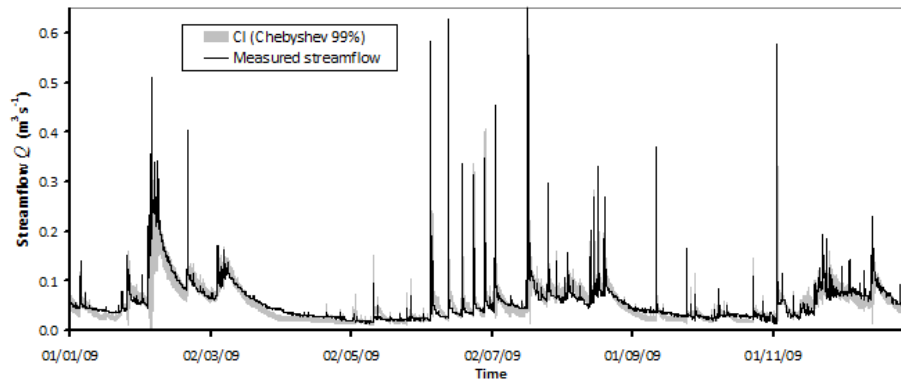
Fig. 9. Measured streamflow against modelled 99% Chebyshev confidence interval (vertical axis truncated at 0.6 \text{ m}^3 \text{ s}^{-1} ).
