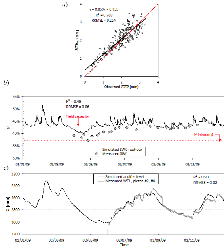
Fig. 8. Validation of: (a) daily evapotranspiration ETR_m , (b) soil water content \theta at the 1.6 m root-reservoir and (c) water table level z ( R^2 : determination coefficient, RRMSE: relative root mean squared error).
