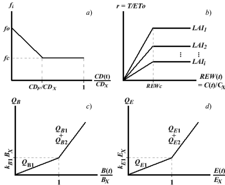
Fig. 4. (a) Infiltration from surface reservoir as a function of soil water content in non-saturated reservoirs. (b) The ratio r = T/ET_0^{-1} as a function of relative extractable water REW and for different values of LAI (here, LAI_1 > LAI_2 > \dots > LAI_i ), (c) Surface runoff from the surface reservoir as a function of its water content, (d) Baseflow from the aquifer reservoir as a function of its water content.
