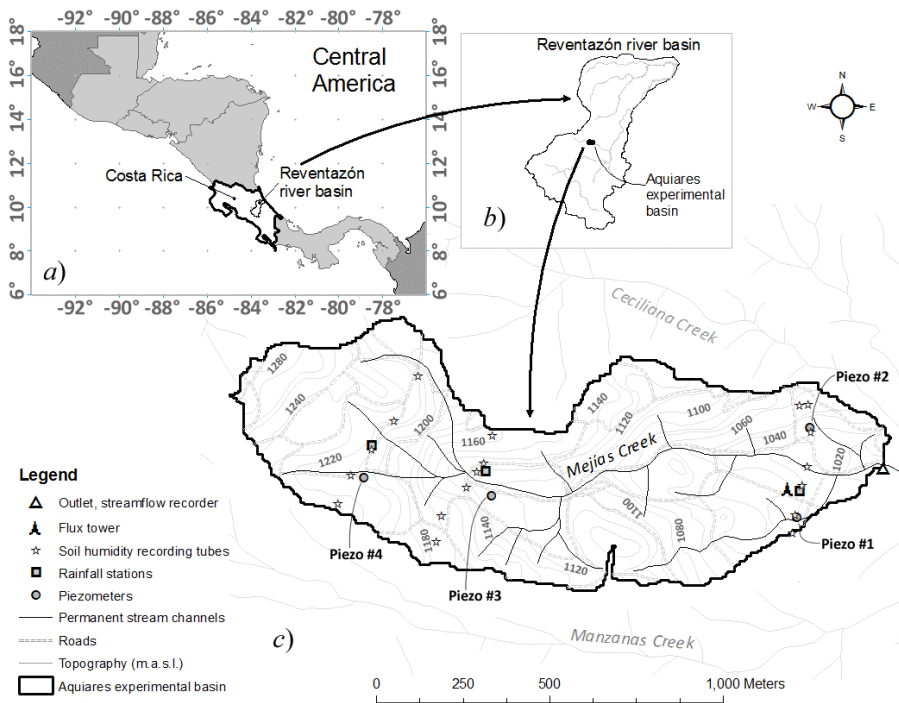
Fig. 1. (a) Location of Reventazón river basin in Costa Rica, Central America. (b) Position of experimental basin inside of Reventazón basin. (c) The “Coffee-Flux” experimental basin in Aquires farm and its experimental setup to measure the water balance components.
