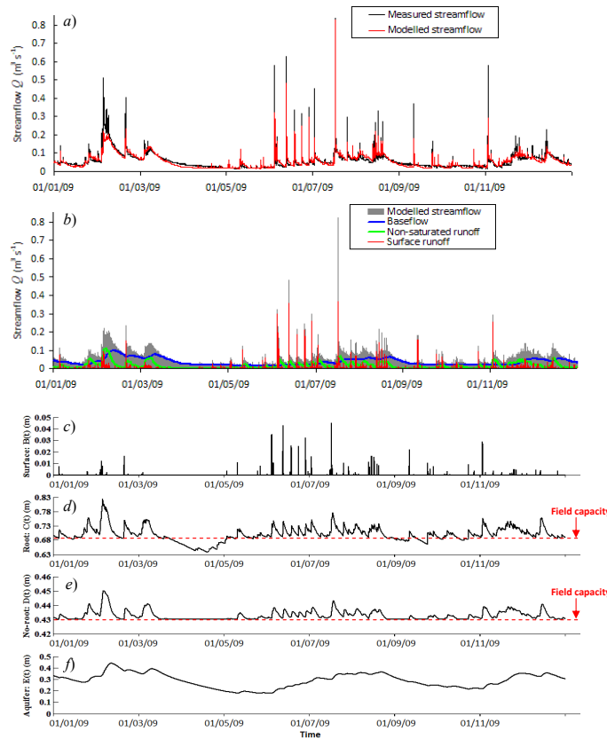
Fig. 7. Model results: (a) measured vs. modelled streamflow, (b) modelled streamflow components. Water level in the model reservoirs: (c) surface reservoir, (d) non-saturated root reservoir (offset by \theta_r C_H to show the absolute water content in the soil layer), (e) non-saturated non-root reservoir (offset by \theta_r D_H ) and (f) aquifer reservoir.
