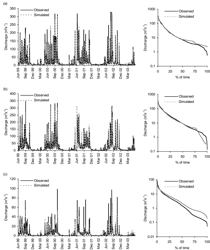
Fig. 2. Comparison (daily flows and flow duration curves) of observed and simulated discharge for the three modelled sub-catchments (June 1999–May 2003) (a) Thoubal, (b) Iril, (c) Nambul.
