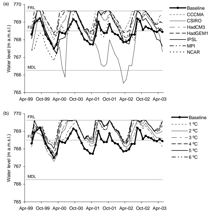
Fig. 9. Simulated mean monthly Loktak Lake water levels (June 1999–May 2003) (a) Group 1 scenarios, (b) Group 2 scenarios (FRL: full reservoir level, FL: flood level, MDL: minimum drawdown level).
