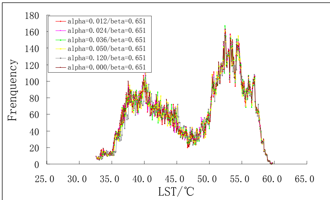
AC-Fig. 3a The sensitivity of our used LST retrieval method to alpha parameter.
