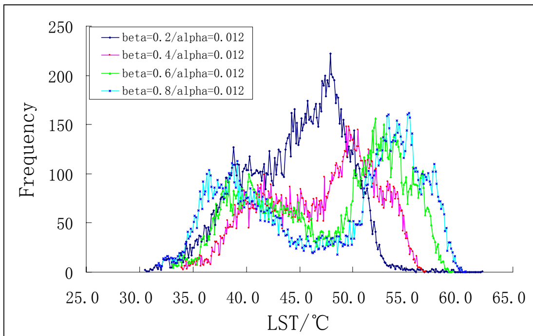
AC-Fig. 3b The sensitivity of our used LST retrieval method to beta parameter.
