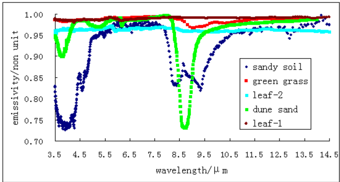
AC-Fig. 2. The emissivity spectrums of five selected materials from MODIS/ASTER emissivity spectral library
