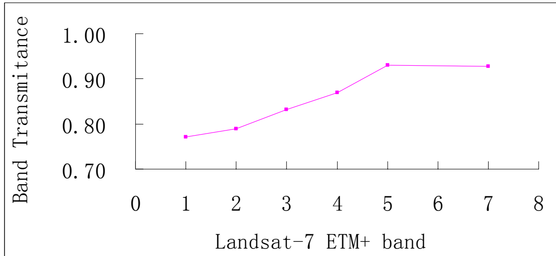
AC-Fig. 1 Landsat-7 ETM+ band transmittance computed using 6S model
